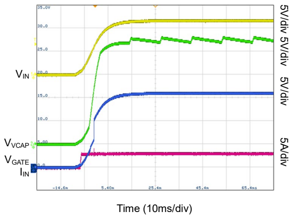
V_{VCAP} During Start-Up, 3A Load
