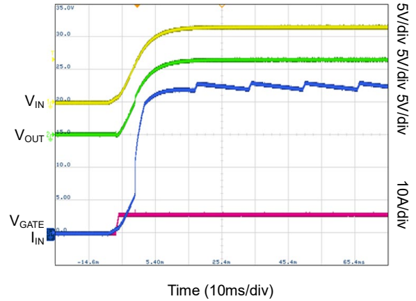
Start-Up, 5.8A Load
