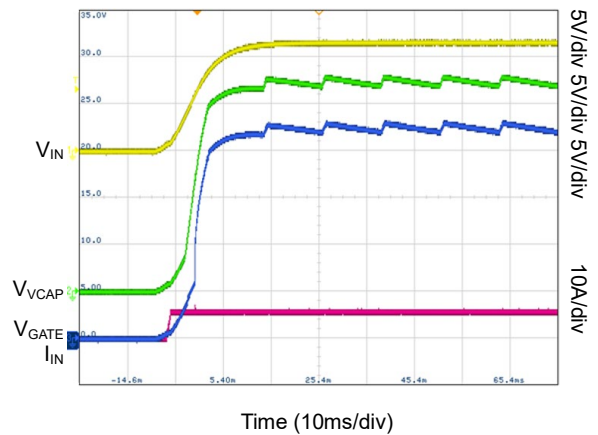
V_{VCAP} During Start-Up, 5.8A Load
