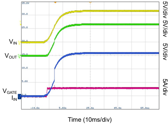
Start-Up, 3A Load
