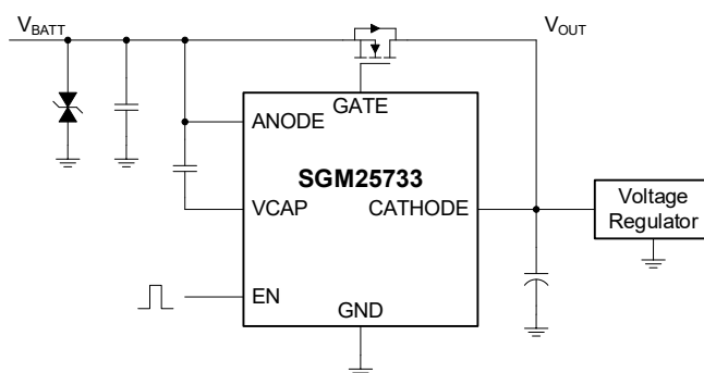
Figure 1. Application Schematic
