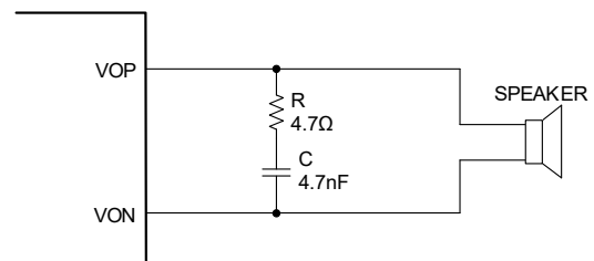
Figure 8. RC Snubber Circuit
