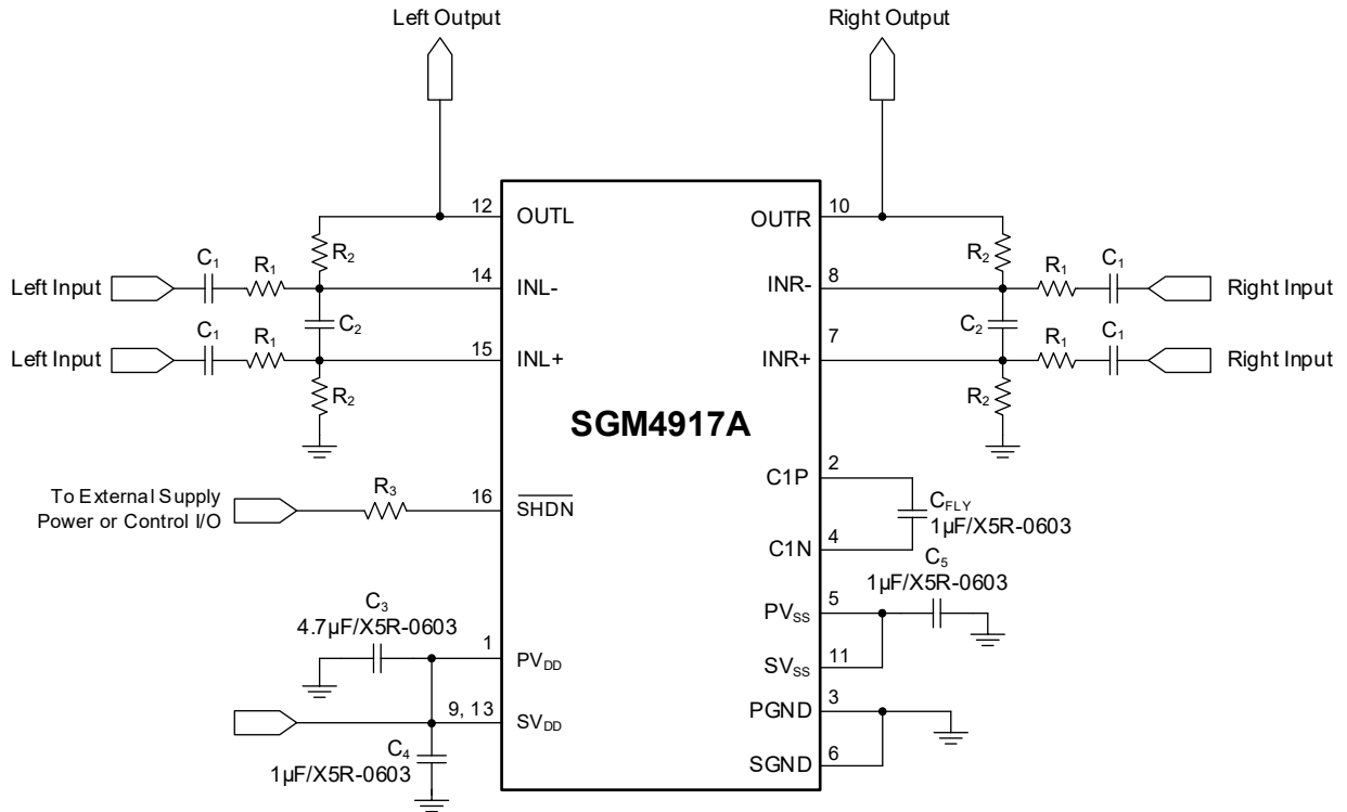
Figure 3. SGM4917A Differential Input Application Circuit
