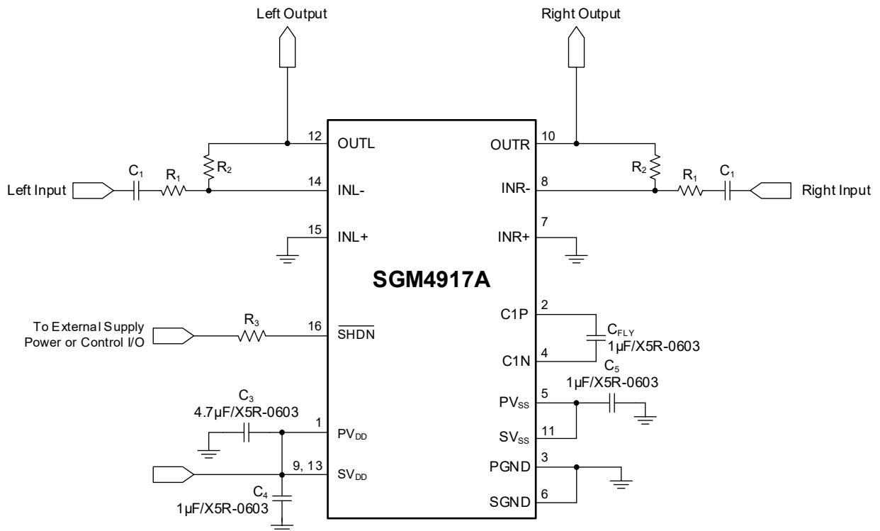
Figure 4. SGM4917A Single-Ended Input Application Circuit
