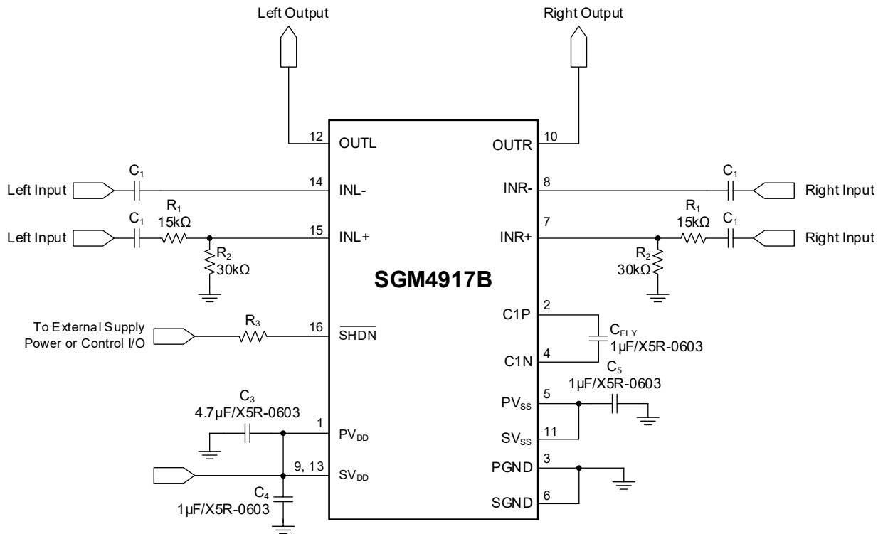
Figure 5. SGM4917B Differential Input Application Circuit
