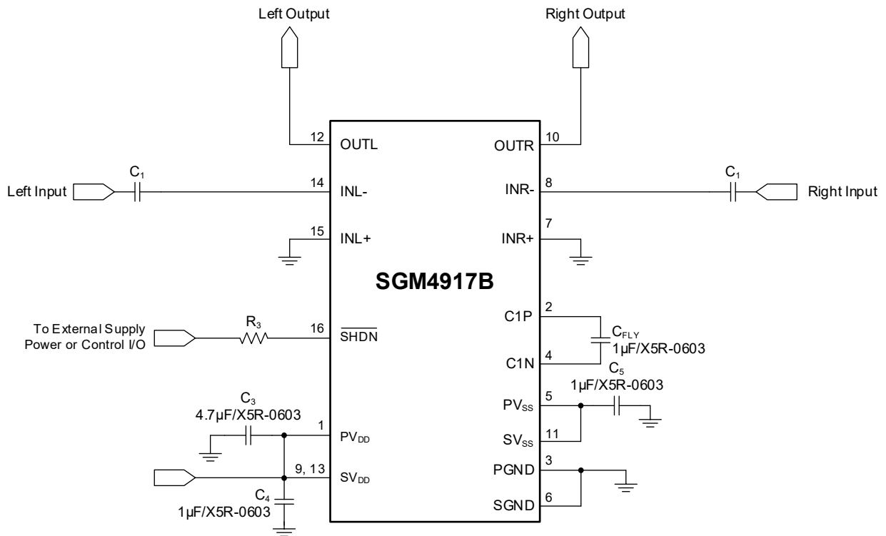
Figure 6. SGM4917B Single-Ended Input Application Circuit
