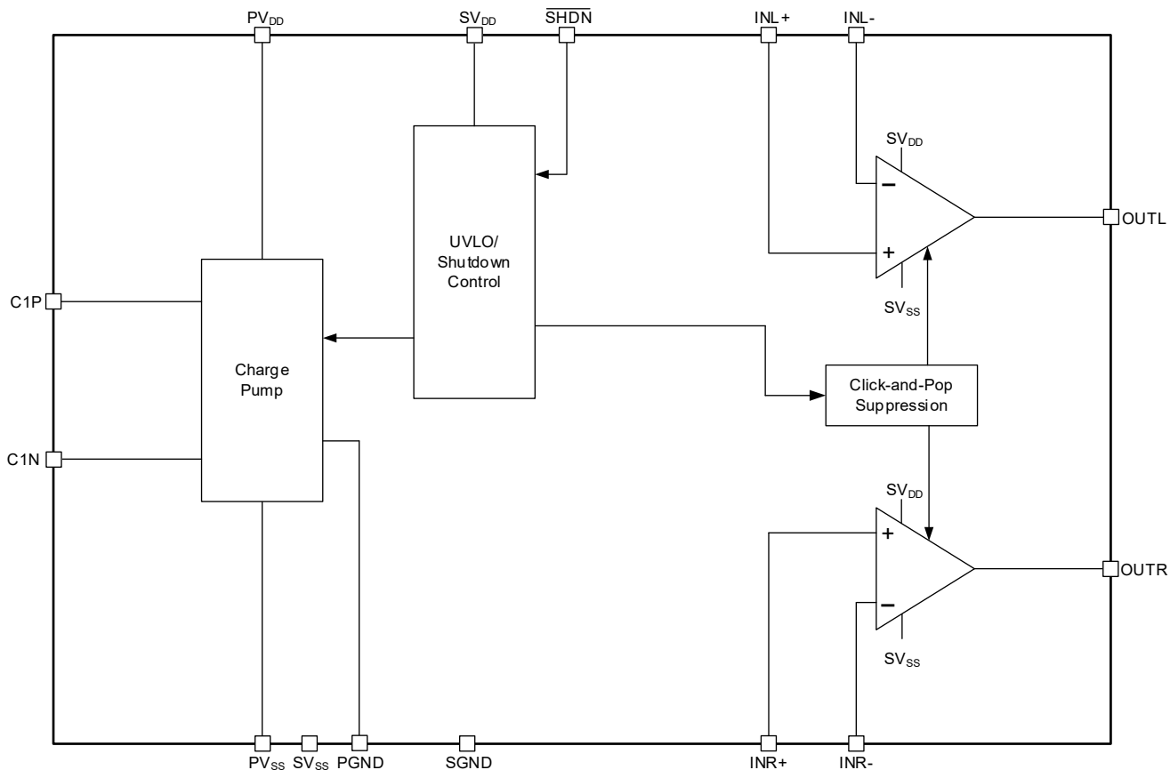
Figure 1. SGM4917A Block Diagram
