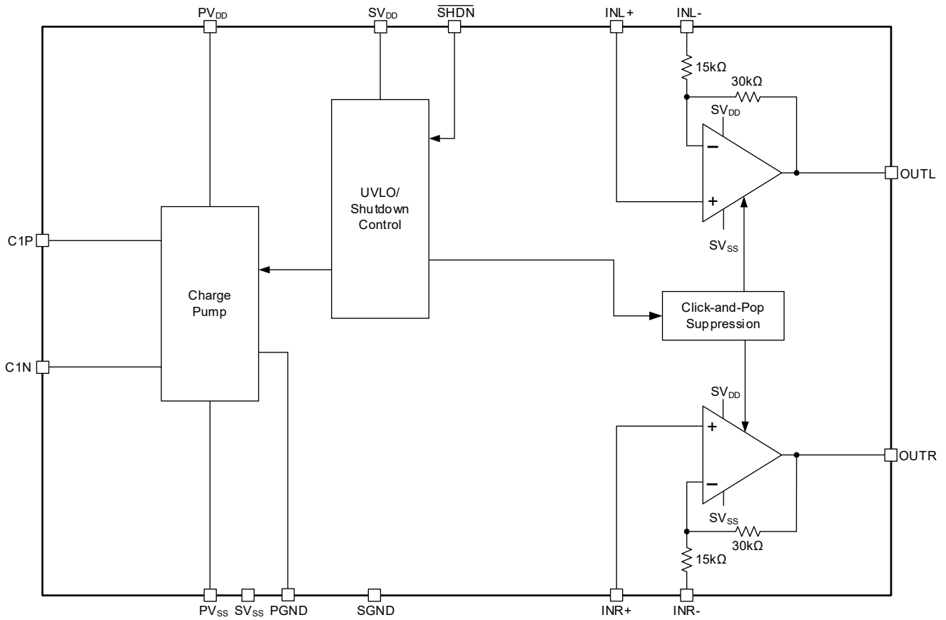
Figure 2. SGM4917B Block Diagram
