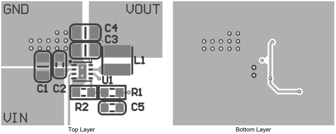
Figure 11. PCB Layout
