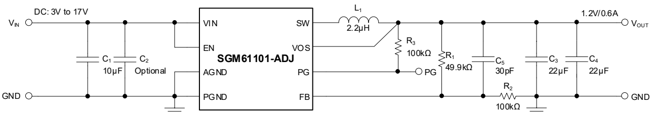
Figure 6. 1.2V Output Voltage Application of SGM61101-ADJ
