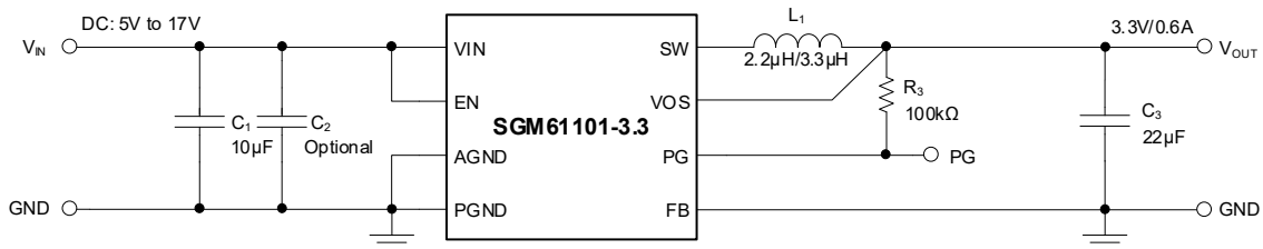
Figure 9. Application of SGM61101-3.3
