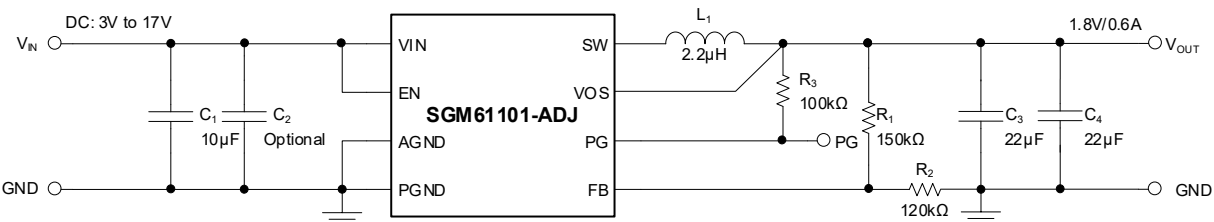
Figure 7. 1.8V Output Voltage Application of SGM61101-ADJ
