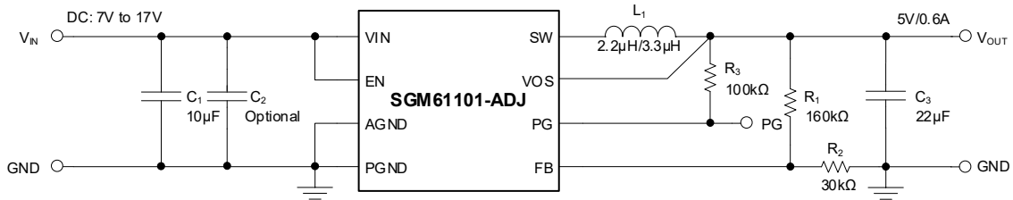
Figure 8. 5V Output Voltage Application of SGM61101-ADJ
