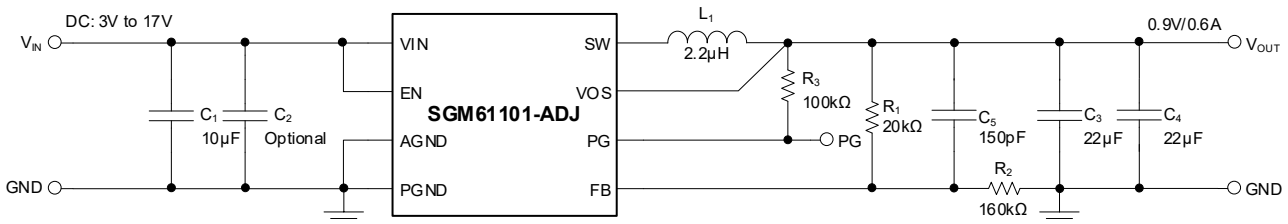
Figure 5. 0.9V Output Voltage Application of SGM61101-ADJ
