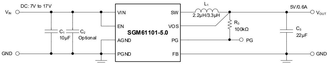
Figure 10. Application of SGM61101-5.0
