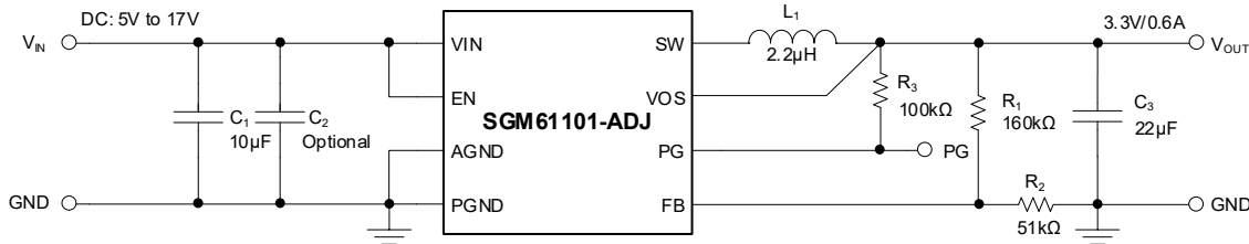
Figure 4. 3.3V Output Voltage Application of SGM61101-ADJ
