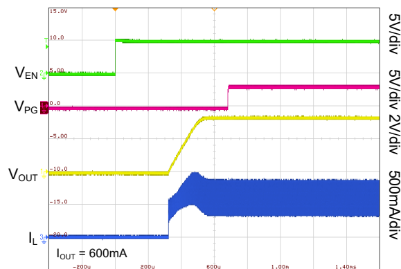
Startup with 600mA
