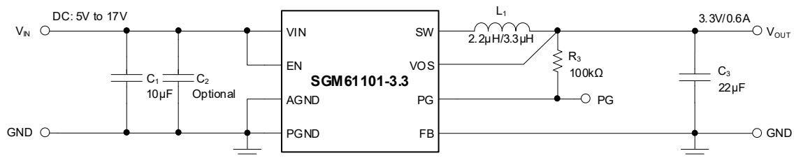
Figure 9. Application of SGM61101-3.3
