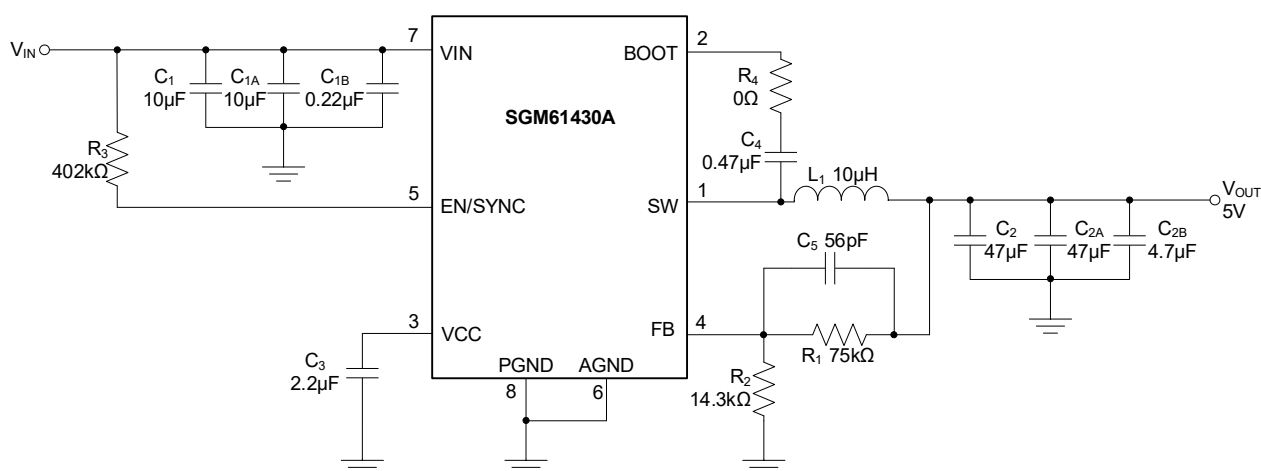
Figure 9. SGM61430A Basic Application Schematic
