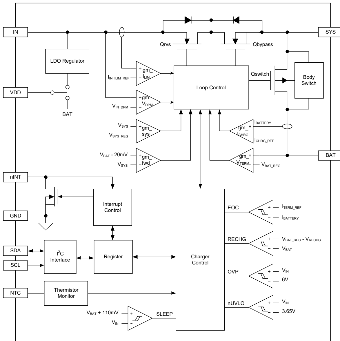
Figure 2. Block Diagram
