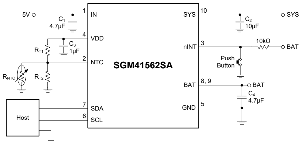
Figure 12. SGM41562SA Typical Application Circuit with 5V Input
