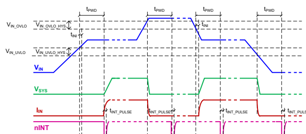
Figure 4. Input Power Detection and nINT Signaling Timings
