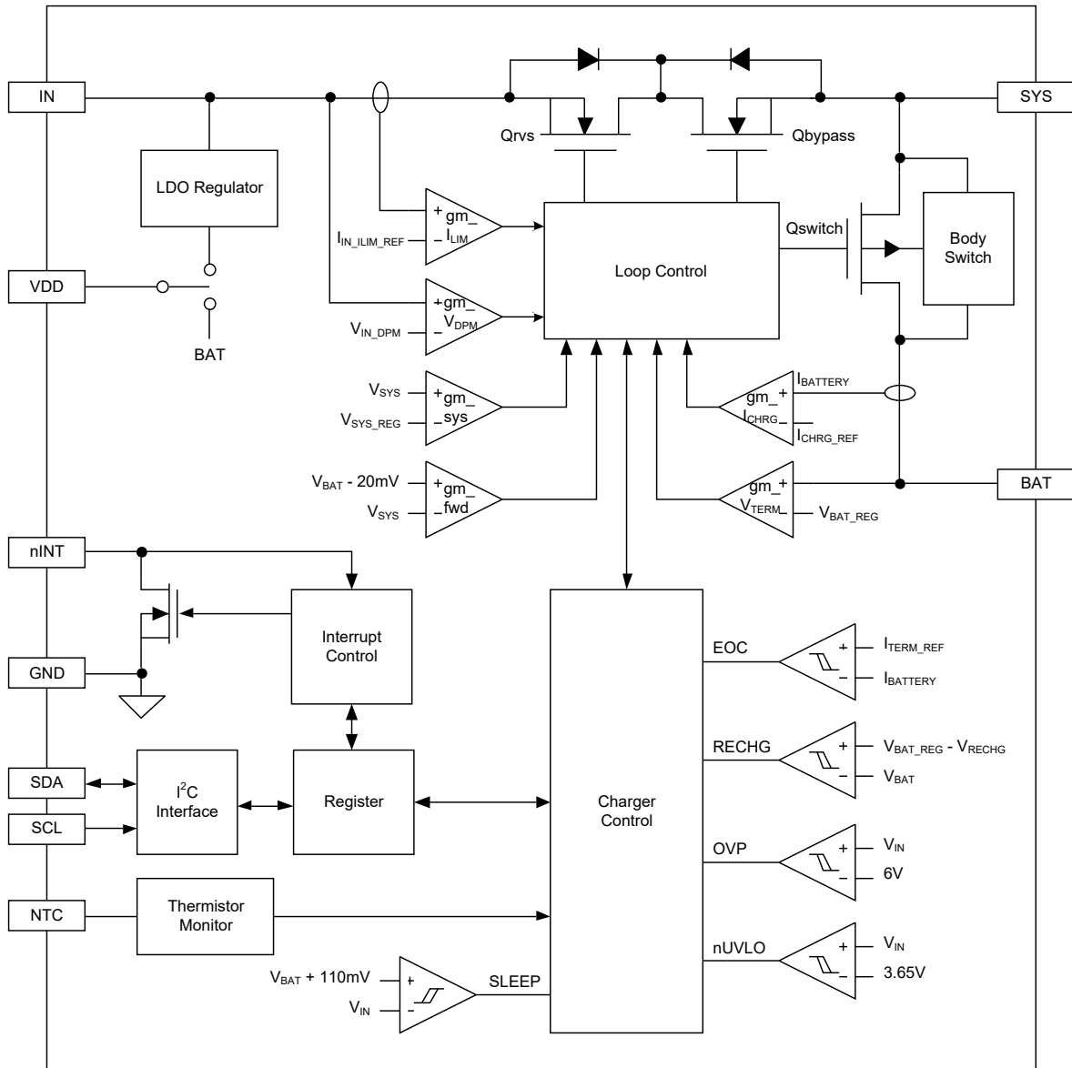
Figure 2. Block Diagram
