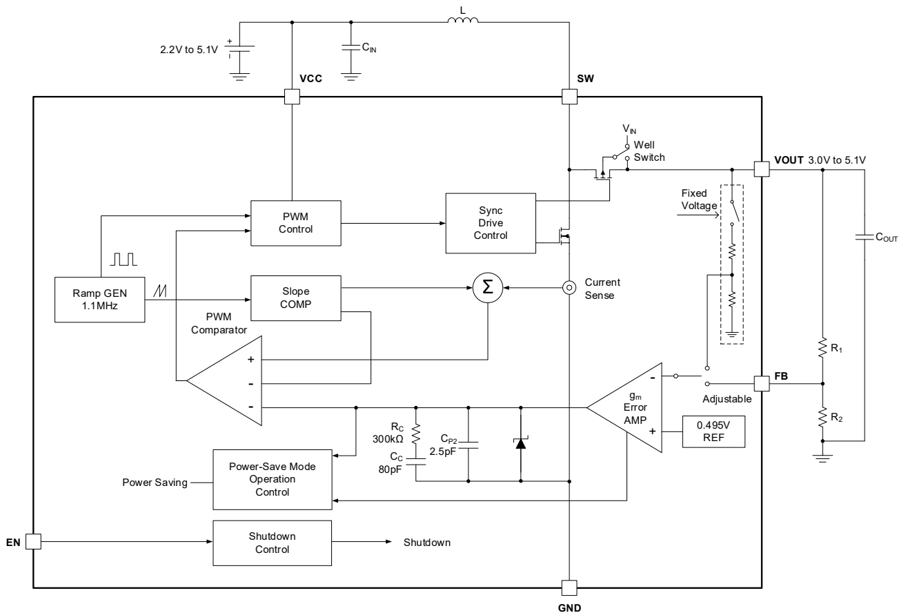
Figure 4. Block Diagram
