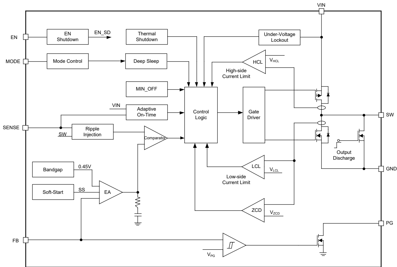
Figure 2. Block Diagram
