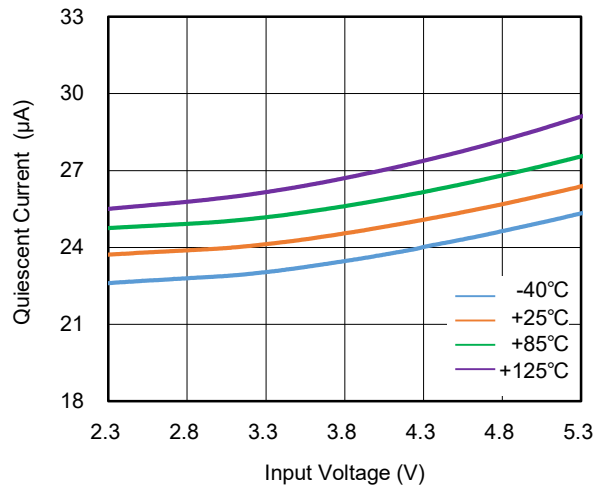
Quiescent Current vs. Input Voltage in PSM
