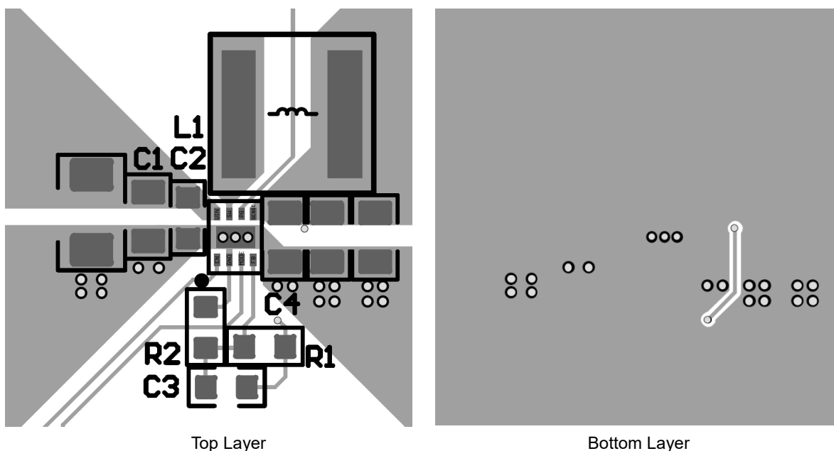
Figure 4. PCB Layout
