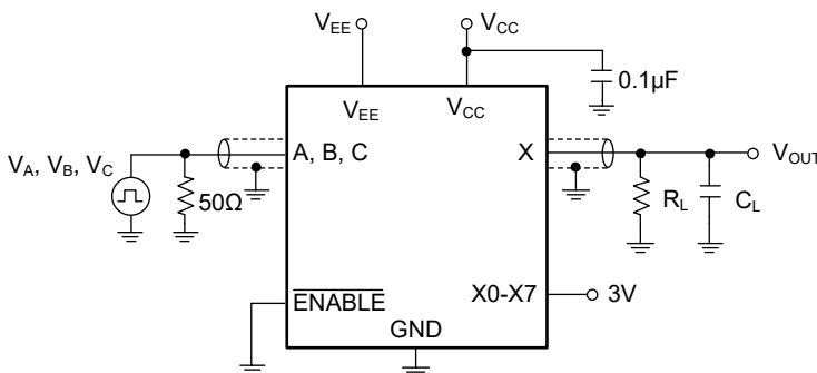
Test Circuit 3. Break-Before-Make Delay Time ( t_D )
