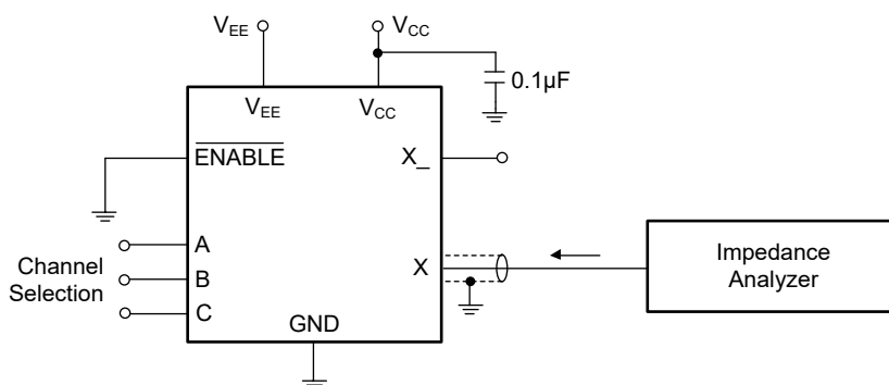
Test Circuit 7. Capacitance
