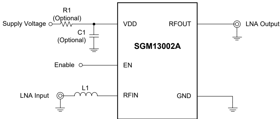
Figure 2. SGM13002A Typical Application Circuit
