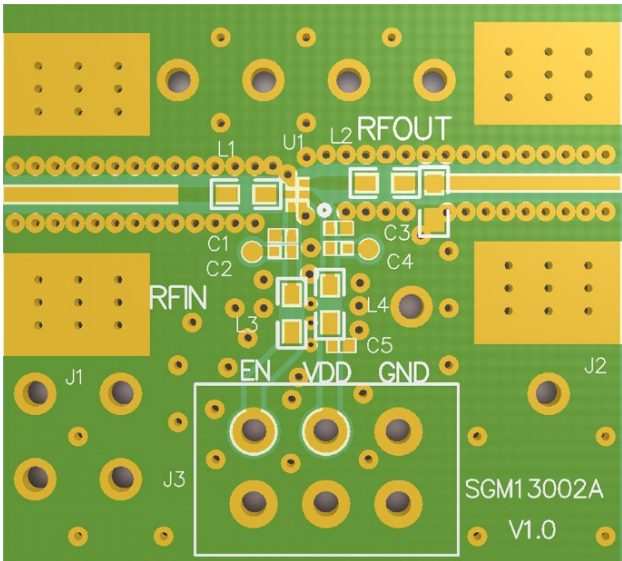
Figure 3. SGM13002A Evaluation Board Layout
