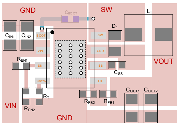
Figure 7. Layout
