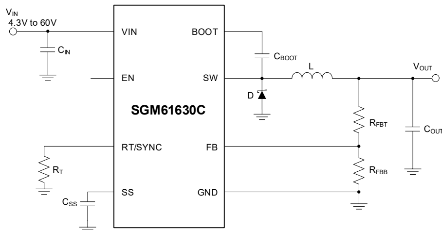
Figure 1. SGM61630C Simplified Schematic
