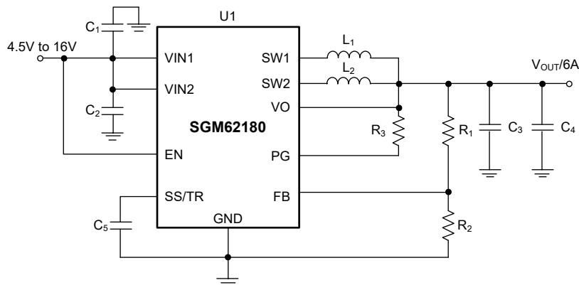
Figure 3. SGM62180 Typical 6A Converter with 4.5V to 16V Input
