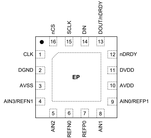
TQFN-3.5x3.5-16L
