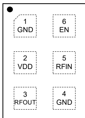
UTDFN-1.1×0.7-6L
