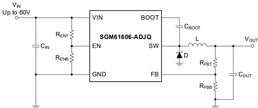
Figure 1. Simplified Schematic
