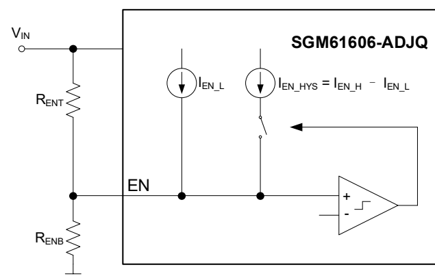
Figure 3. Adjustable VIN Under-Voltage Lockout
