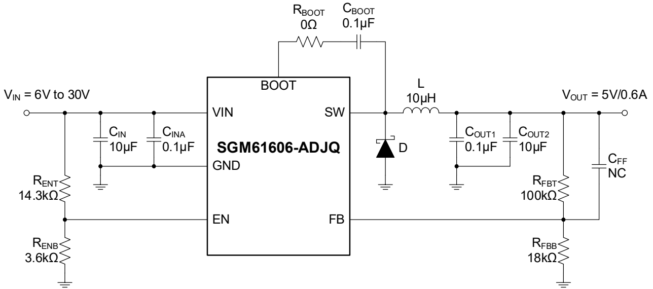
Figure 6. A Reference Design for 5V/0.6A Application
