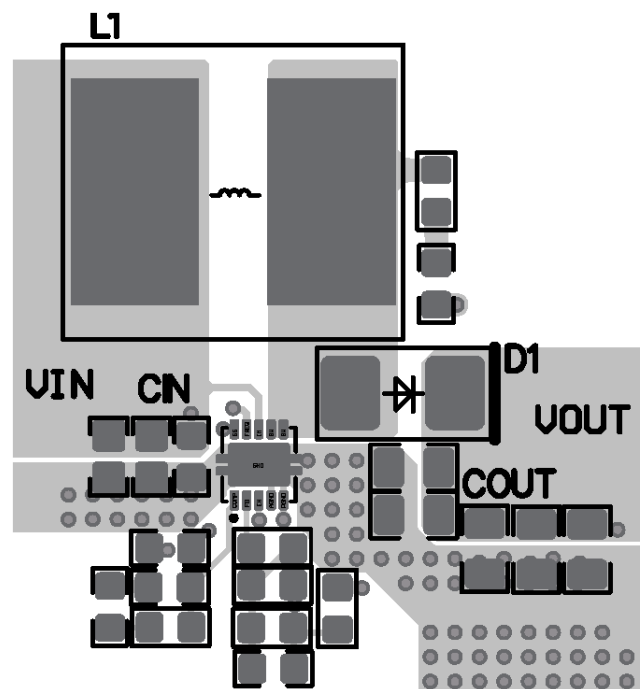
Figure 4. PCB Layout
