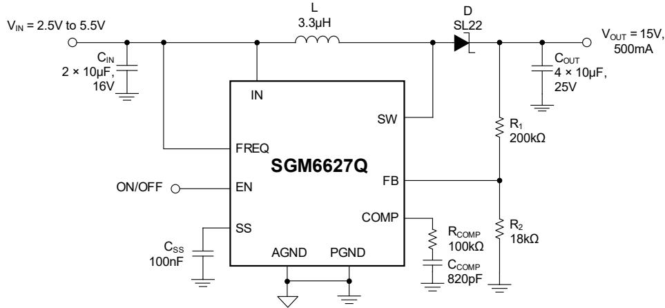
Figure 3. f sw = 1.2MHz, Application Circuit
