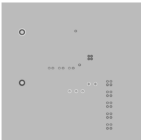
Figure 12. Middle Layer 1
