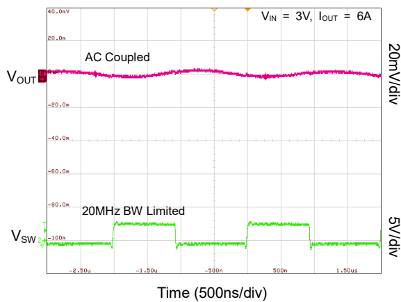
Output Ripple
