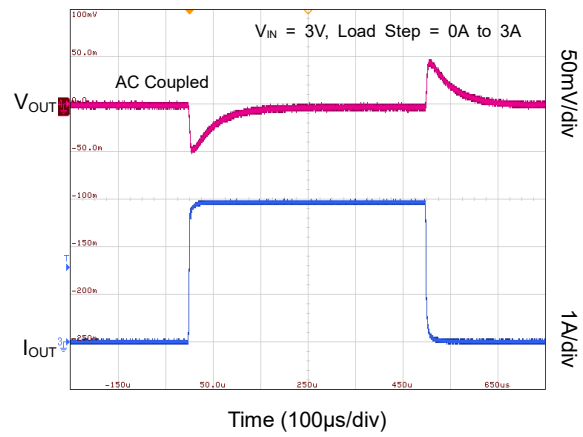
Transient Response
