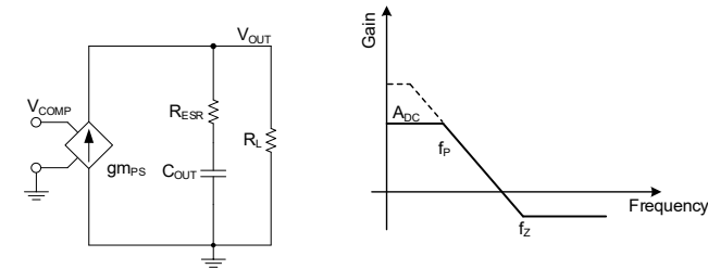
Figure 7. Simplified Model for Peak Current Mode Control and Frequency Response
