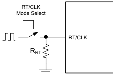
Figure 5. Use RT and CLK Modes Together
