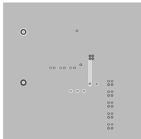
Figure 13. Middle Layer 2
