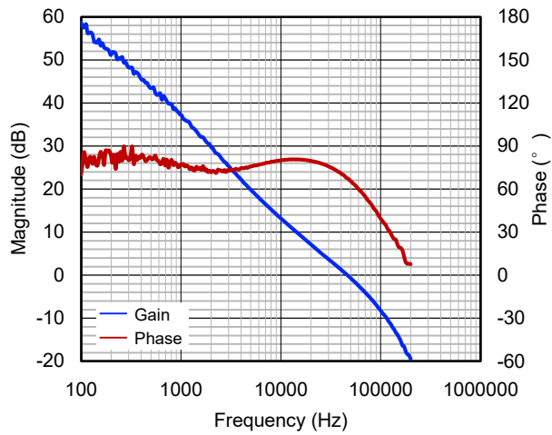
Loop Response
