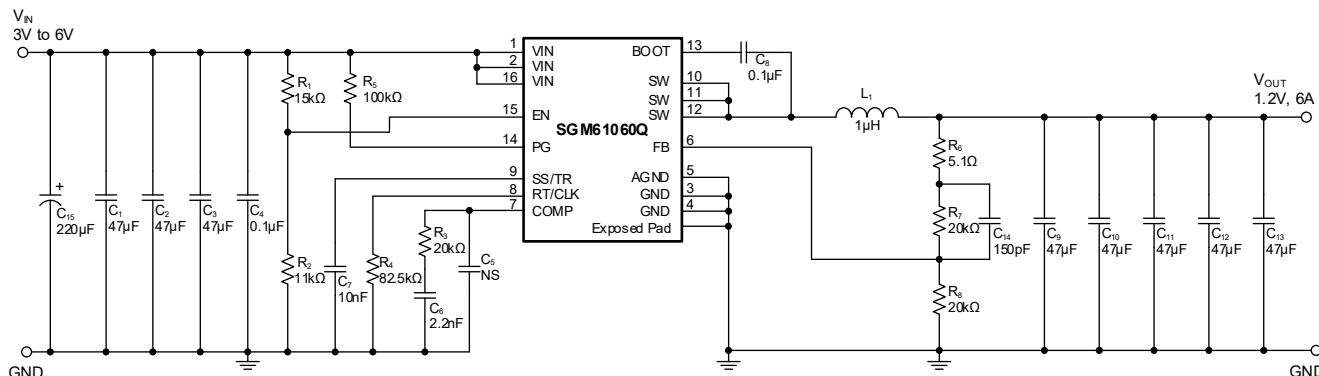
Figure 9. SGM61060Q Typical Application Circuit
