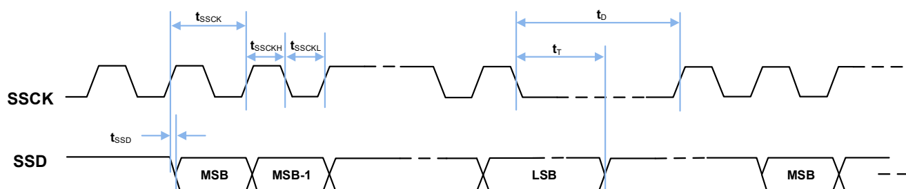
Figure 24. SSI Timing
