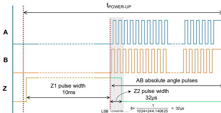
Figure 11. Power-Up Angular Output Signal of Pulse Sequence 3
