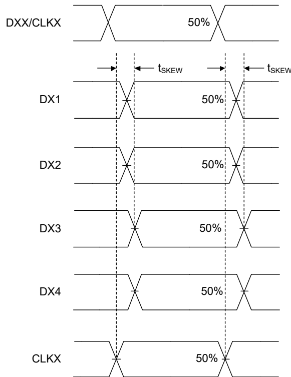
Test Circuit 9. Channel-to-Channel Skew ( t_{SKEW\_INTER} )
