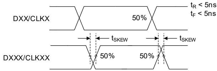
Test Circuit 8. Opposite Transitions of Same Output ( t_{SKEW\_INTRA} )
