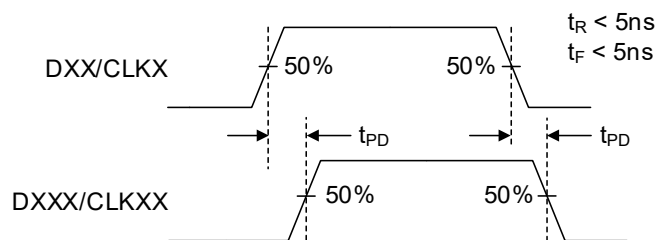
Test Circuit 10. Propagation Delay Time ( t_{PD} )
