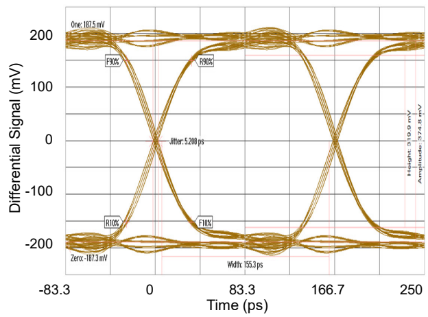
6Gbps (200mV PP ), After Switch
