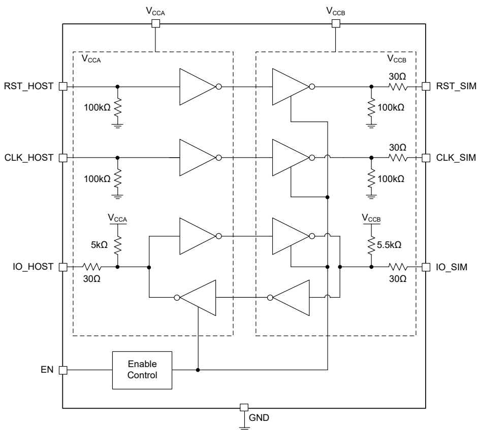
Figure 3. Block Diagram
