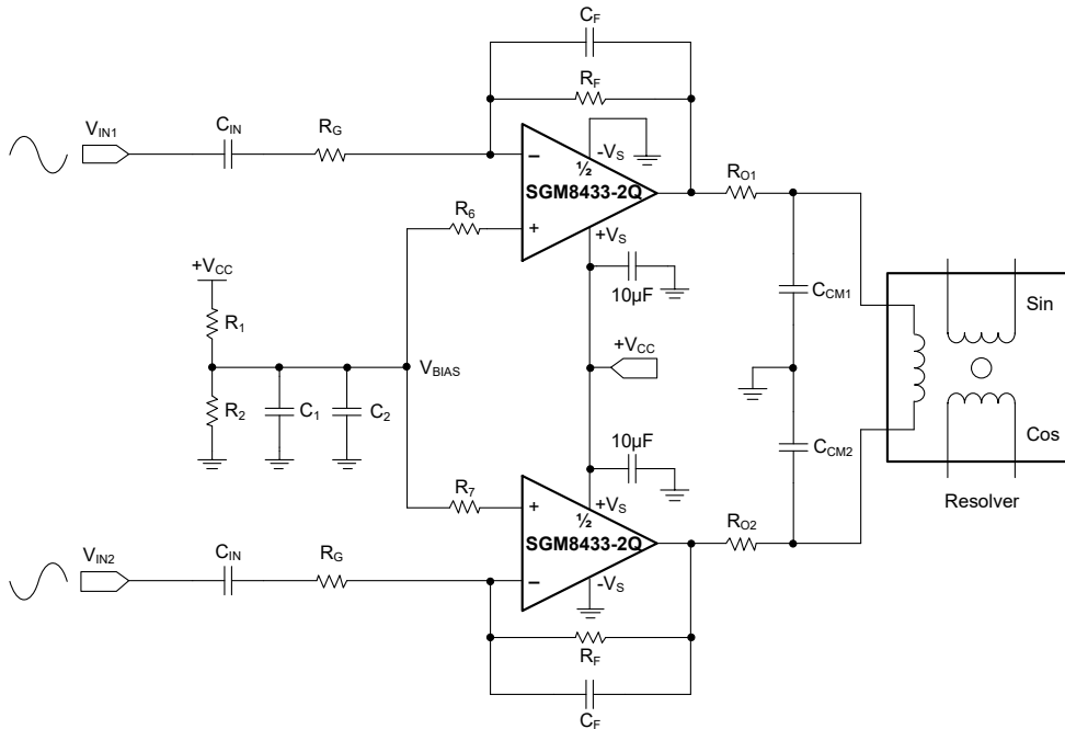
Figure 8. Simplified Resolver Excitation Circuit without SGM8212-1Q
