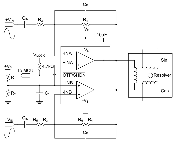
Figure 1. Simplified Schematic for Differential Input
