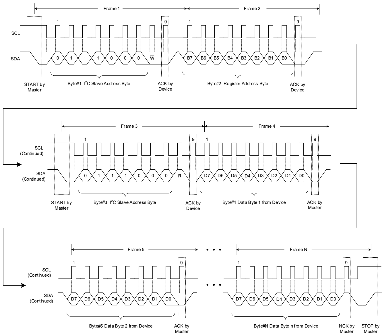
Figure 13. A Multi-Read Transaction
