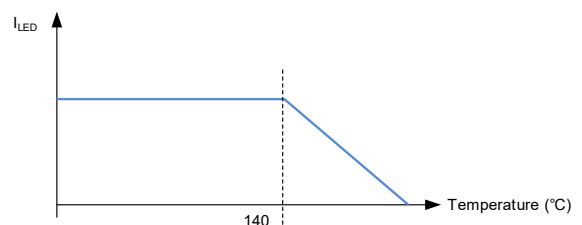
Figure 5. I_{\text{LED}} Decrease with Temperature
