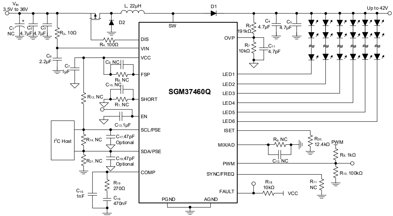
Figure 14. Typical Application Circuit
