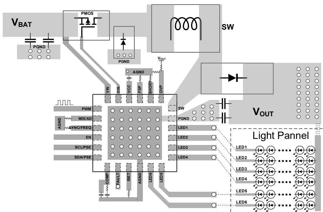
Figure 15. PCB Layout
