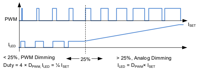
Figure 3. Mix Dimming with 25% Transfer Point
