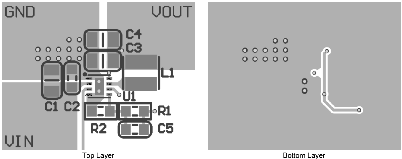
Figure 12. PCB Layout
