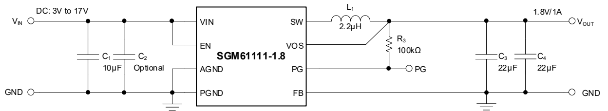
Figure 9. Application of SGM61111-1.8
