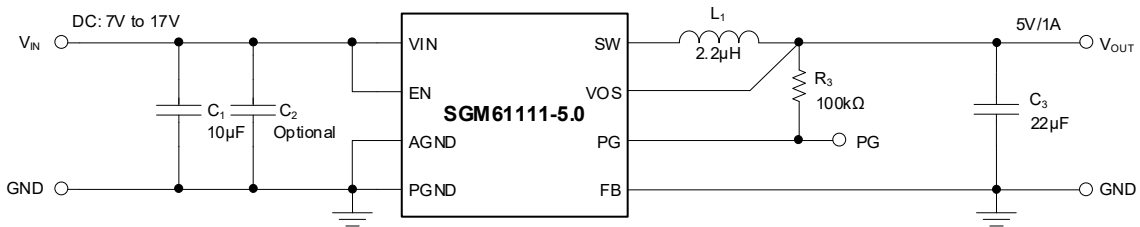
Figure 11. Application of SGM61111-5.0
