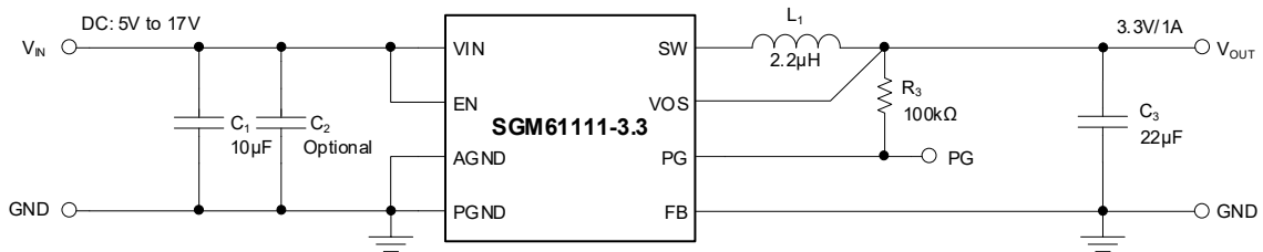
Figure 10. Application of SGM61111-3.3
