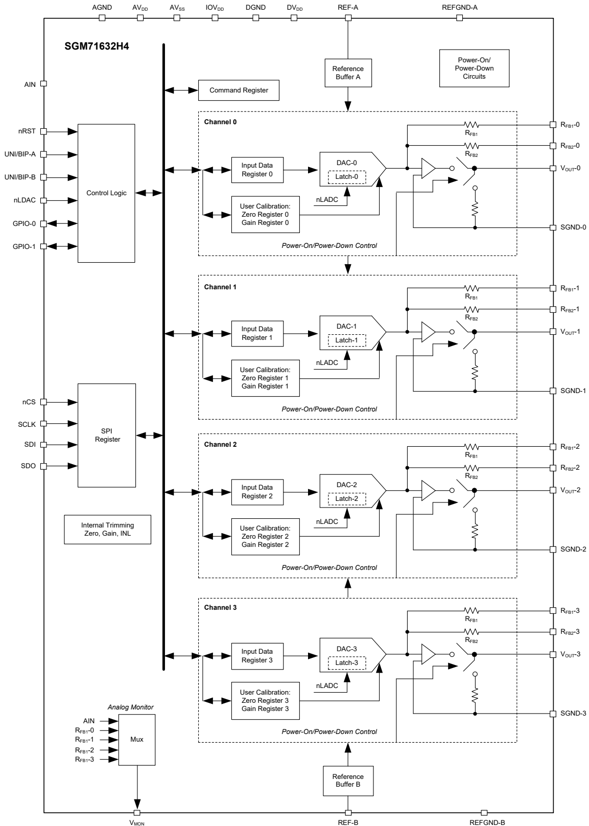
Figure 1. Block Diagram
