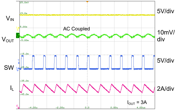
Time (1μs/div)
