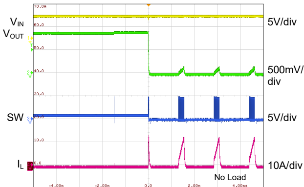
Time (1ms/div)
