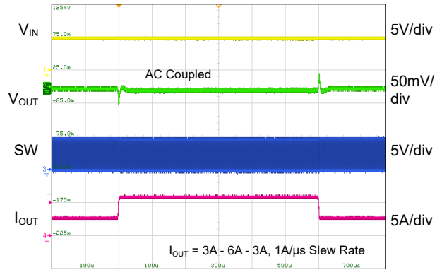
Time (100μs/div)
