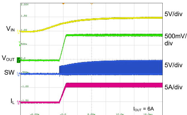
Time (3ms/div)
