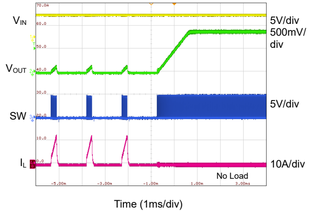
Hiccup with Output Short (FPWM, Recovery)
