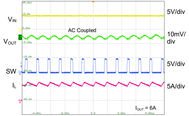
Time (1μs/div)
