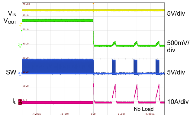
Time (1ms/div)
