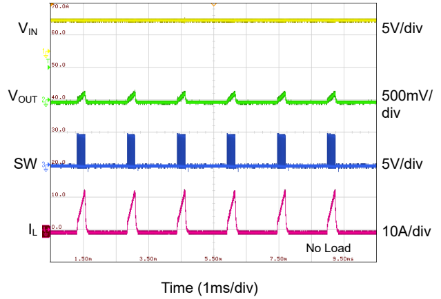
Hiccup with Output Short (FPWM, Steady)
