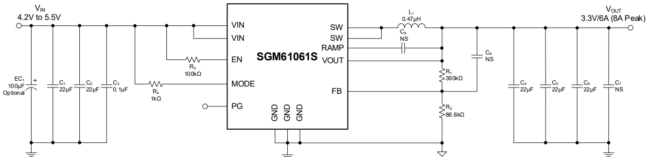
Figure 6. SGM61061S Circuit for 3.3V Output
