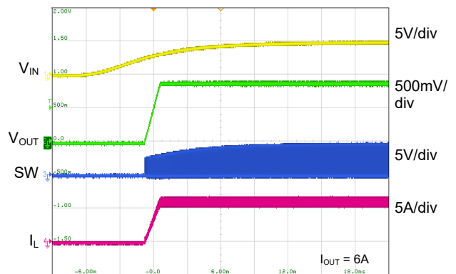
Time (3ms/div)
