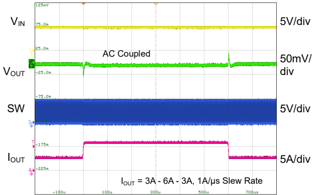
Time (100μs/div)
