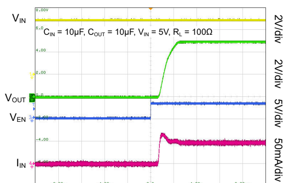
Turn-On Delay and Rise Time
