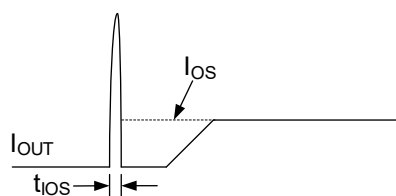
Figure 5. Output Short-Circuit Parameters
