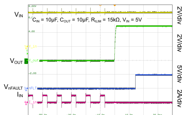
Output Short to No Load Recovery Response
