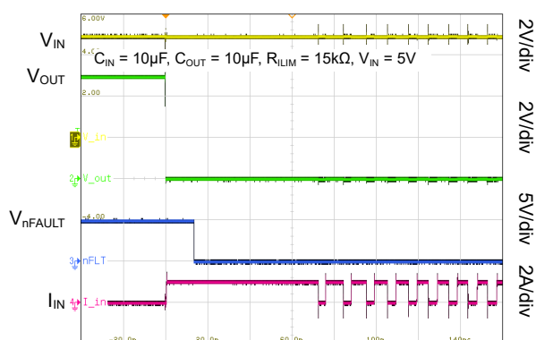
No Load to Output Short Transient Response
