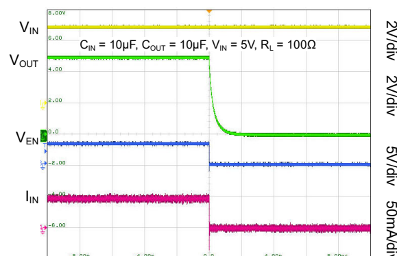
Turn-Off Delay and Fall Time
