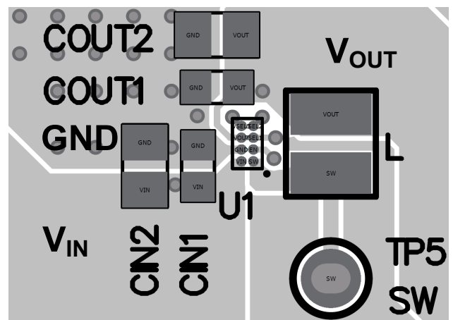
Figure 4. PCB Layout
