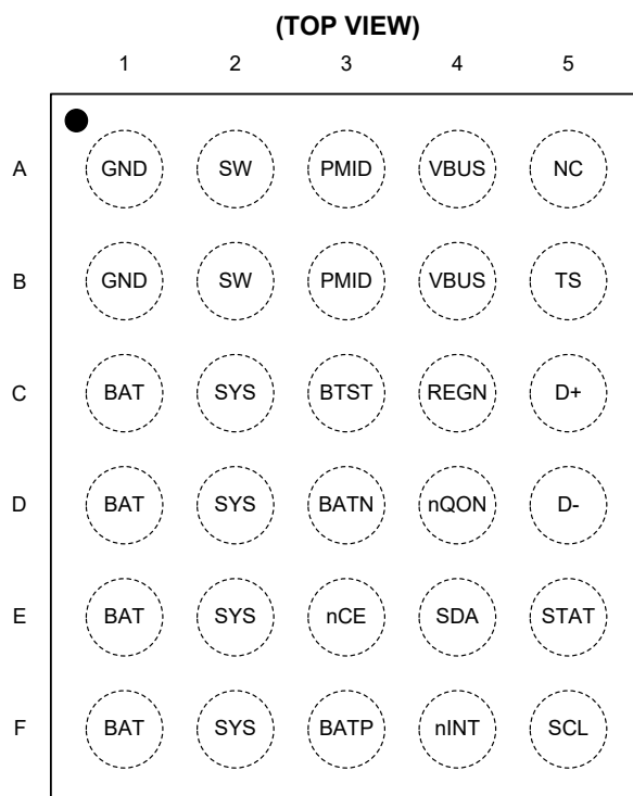
WLCSP-2.05×2.4-30B
