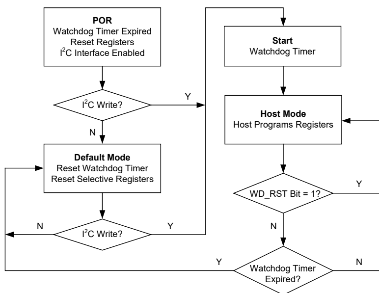
Figure 3. Watchdog Timer Flow Chart
