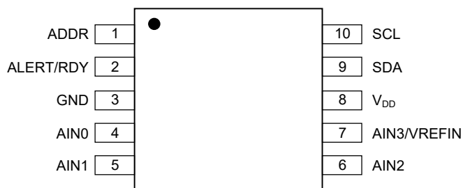
MSOP-10
