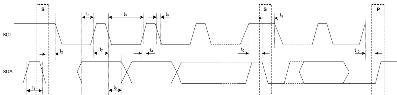
Figure 1. I²C Timing Diagram
