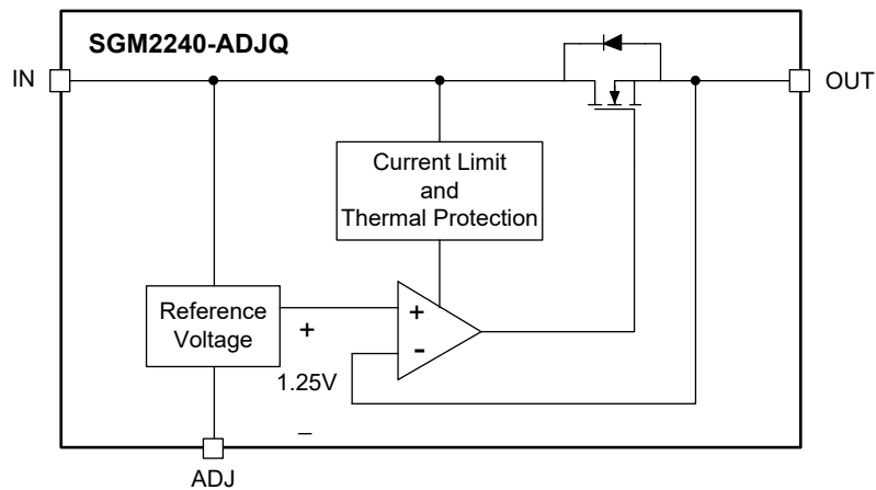
Figure 3. Internal Block Diagram of Adjustable Output Voltage
