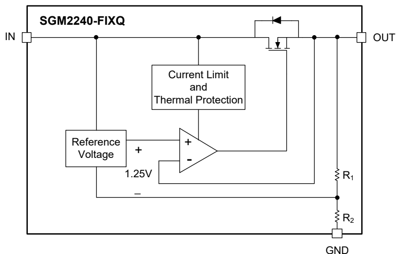
Figure 2. Internal Block Diagram of Fixed Output Voltage
