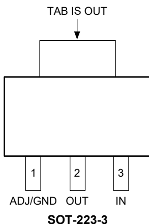
SGM2240xQ (TOP VIEW)
