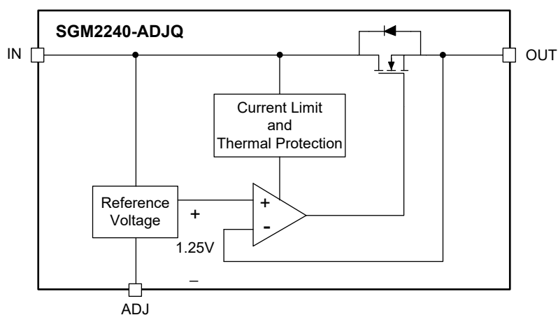
Figure 3. Internal Block Diagram of Adjustable Output Voltage
