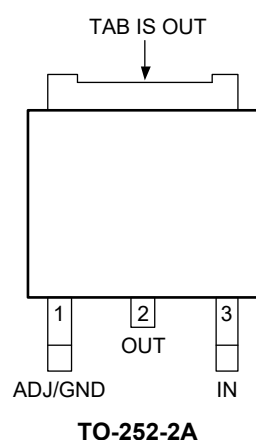
SGM2240xQ (TOP VIEW)
