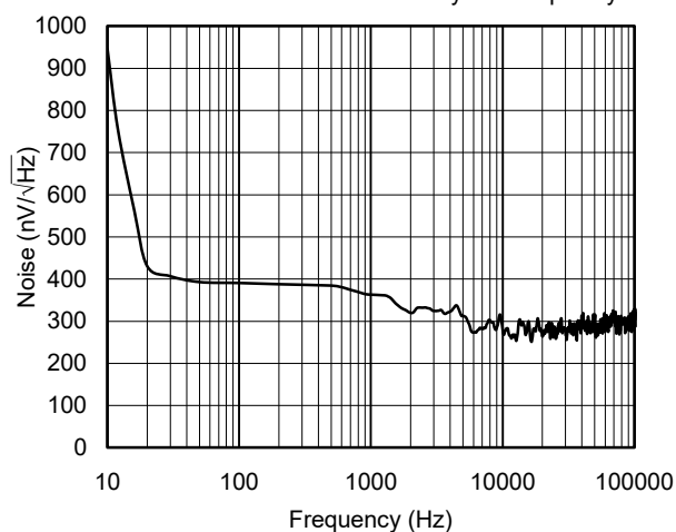
Internal Reference Noise Density vs. Frequency
