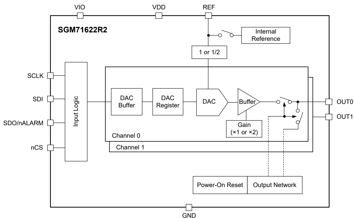
Figure 3. Block Diagram
