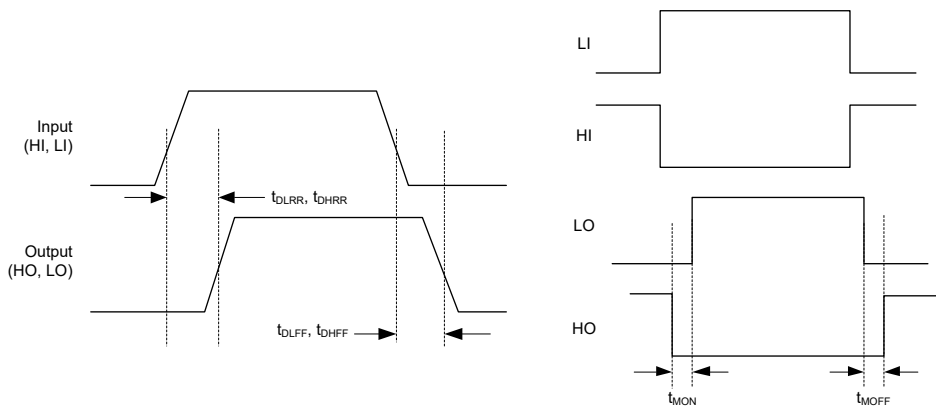
Figure 2. Timing Diagram
