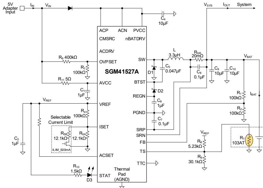
NOTE: USB with 8V input OVP, 900mA or 500mA selectable charge current limit, 0°C to 45°C TS, system connected after sense resistor. Figure 14. Typical Application Schematic with Single-Cell Unremovable Battery
