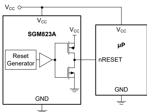
Figure 3. Interfacing to \mu\text{P} with Bidirectional Resets
