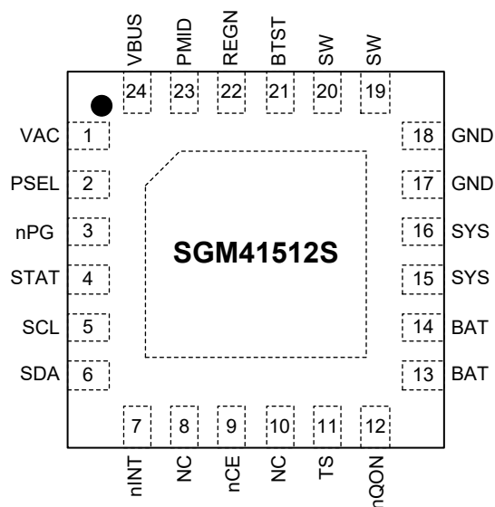
SGM41512S (TOP VIEW)
