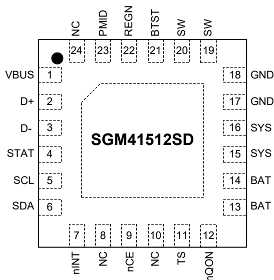
SGM41512SD (TOP VIEW)
