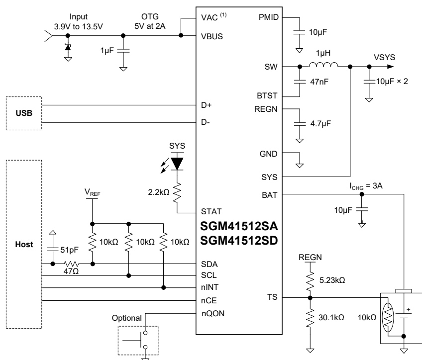
Figure 1. SGM41512S Typical Application Circuit
