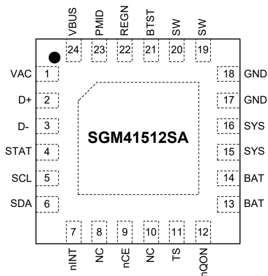
SGM41512SA (TOP VIEW)
