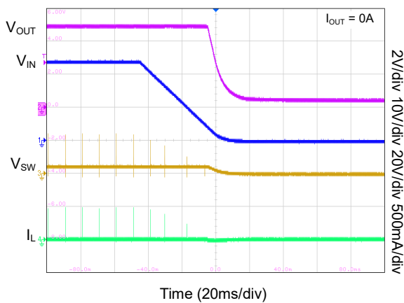
Shutdown by VIN (SGM61610A)
