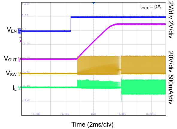
Start-Up by EN (SGM61610B)
