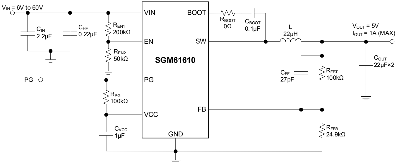
Figure 5. SGM61610 Typical Application Circuit
