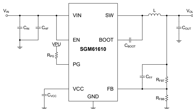
Figure 1. Simplified Schematic
