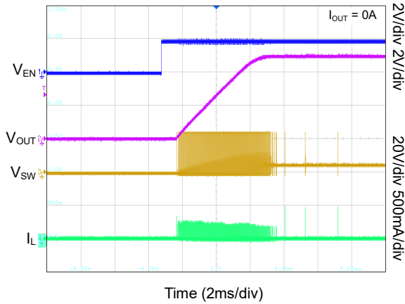
Start-Up by EN (SGM61610A)
