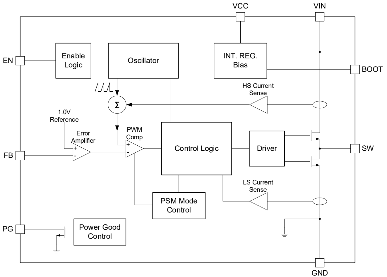
Figure 2. Block Diagram
