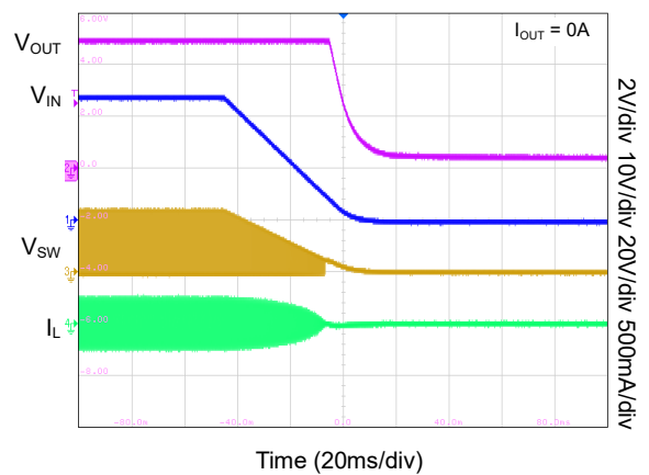
Shutdown by VIN (SGM61610B)
