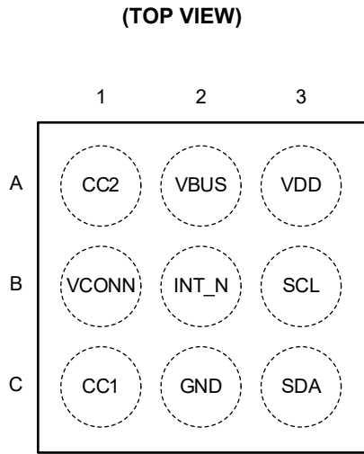
WLCSP-1.17x1.17-9B
