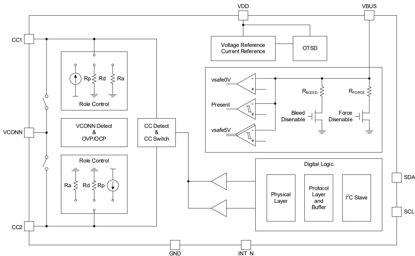
Figure 3. Block Diagram
