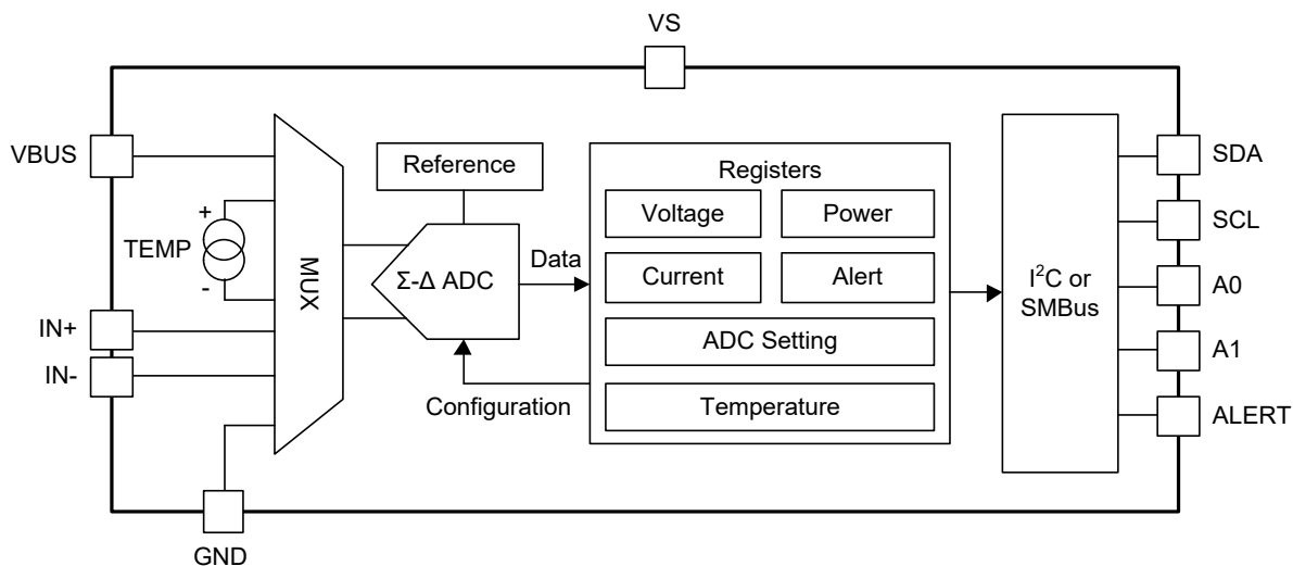
Figure 3. SGM90800A Block Diagram
