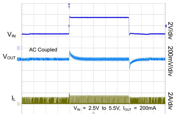
Line Transient Response under Light Load
