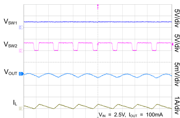
FPWM Switching Waveforms in Boost Mode
