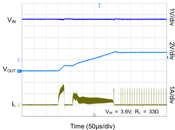
Startup under Light Load
