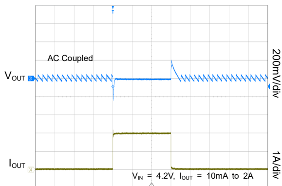
Load Transient Response in Buck Mode
