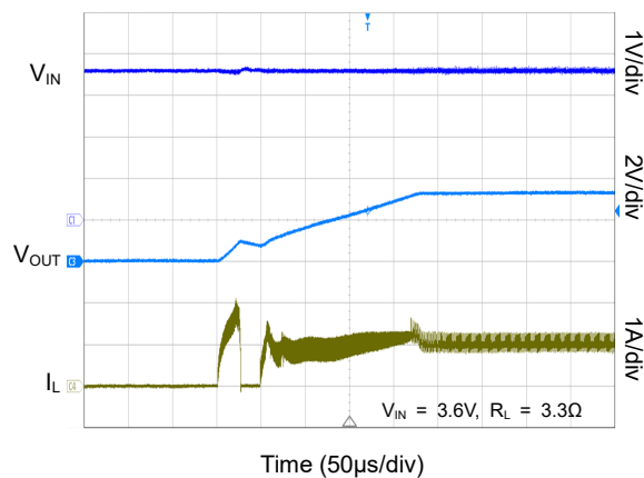
Startup under Heavy Load
