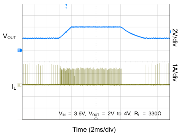
Dynamic Voltage Scaling under PFM
