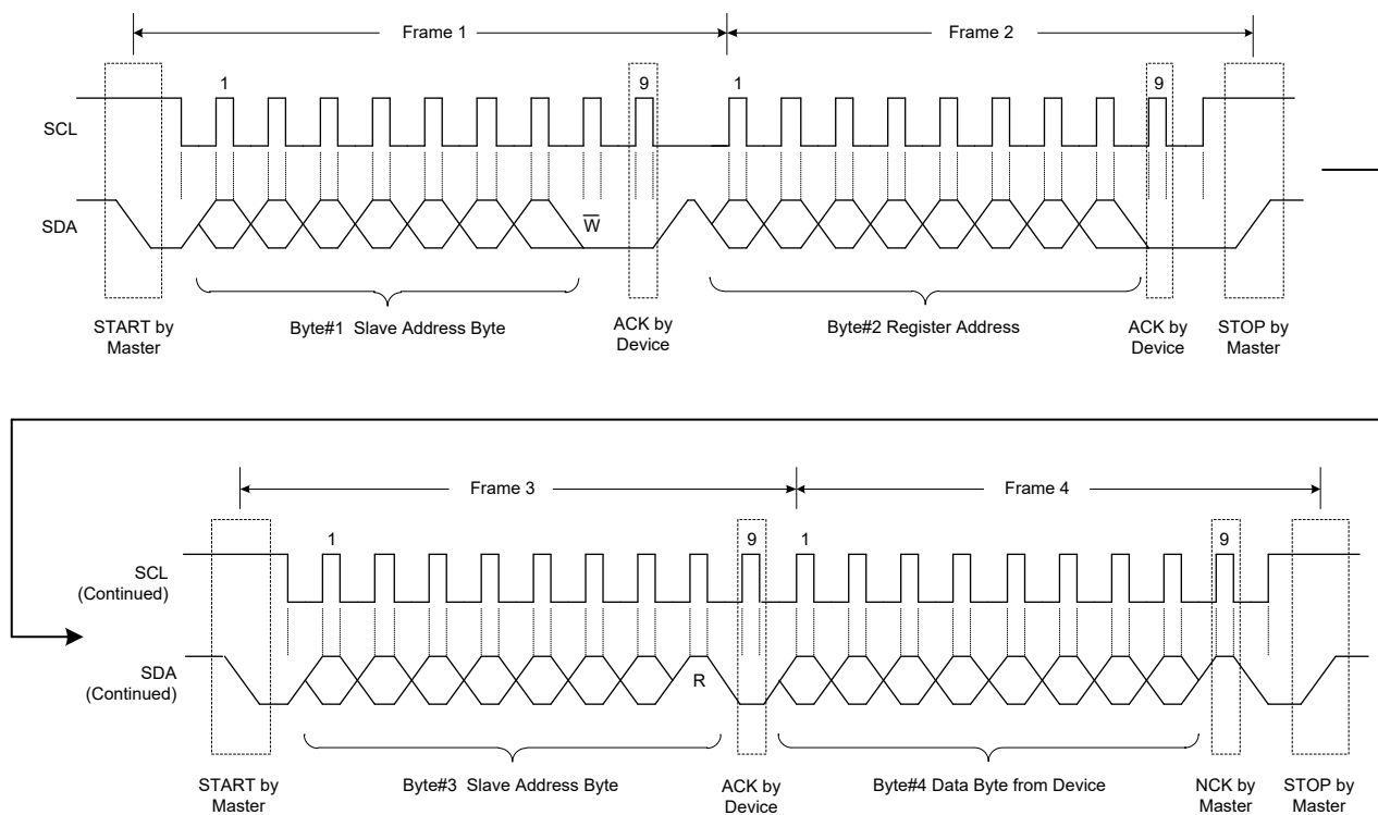
Figure 20. The Format of a READ from a Device Register in the Standard Mode, Fast Mode and Fast Mode Plus
