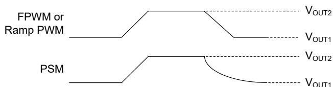
Figure 9. RPWM Operation
