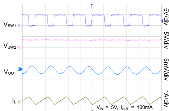
FPWM Switching Waveforms in Buck Mode
