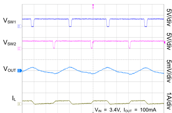
FPWM Switching Waveforms in Buck-Boost Mode
