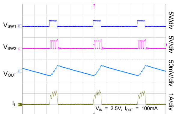
PFM Switching Waveforms in Boost Mode
