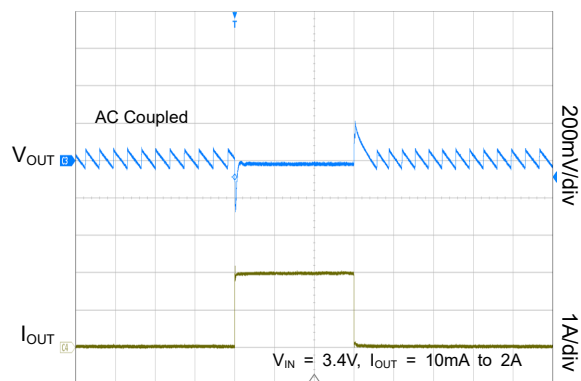
Load Transient Response in Buck-Boost Mode
