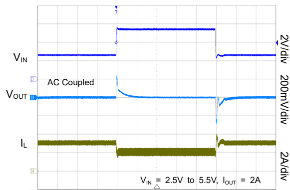
Line Transient Response under Heavy Load
