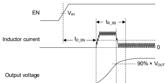
Figure 8. Startup Performance
