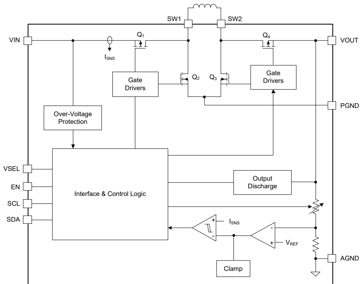
Figure 2. Block Diagram
