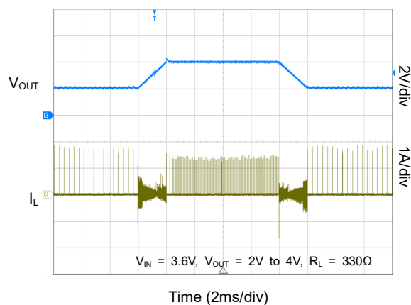
Dynamic Voltage Scaling under RPWM
