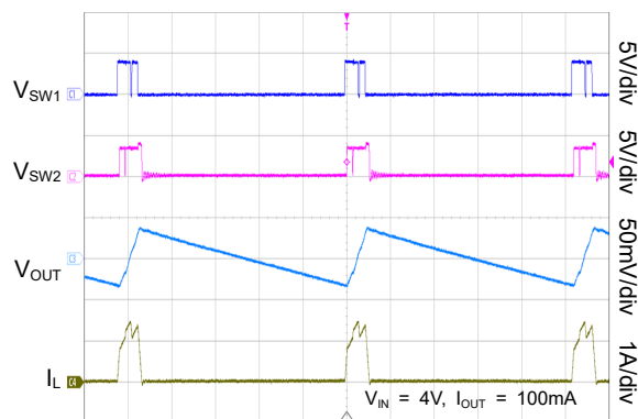
PFM Switching Waveforms in Buck-Boost Mode
