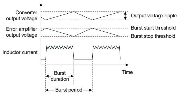
Figure 7. PFM Mode
