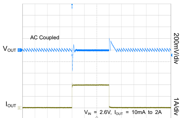
Load Transient Response in Boost Mode
