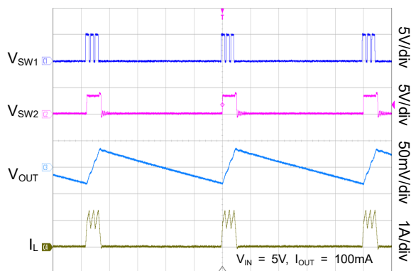
PFM Switching Waveforms in Buck Mode
