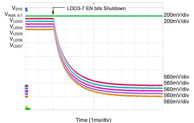
LDO3-7 EN bits Shutdown at I_{LDO3-7} = 0\text{mA}
