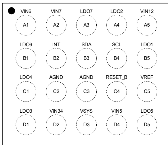
WLCSP-1.83×1.51-20B
