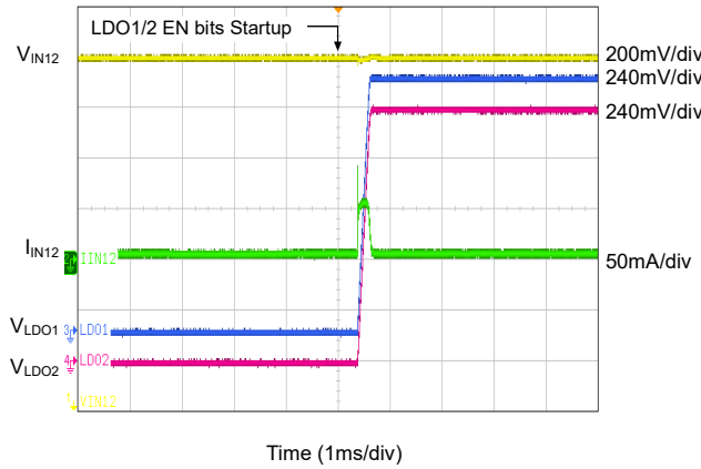
LDO1/2 EN bits Startup at I_{LDO1/2} = 0\text{mA}
