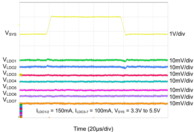
V_{\text{SYS}} Line Transient Response, t_R = t_F = 5\mu\text{s}
