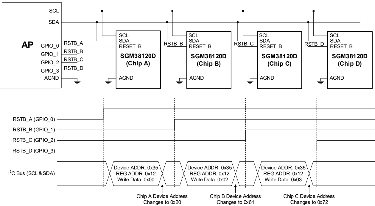
Figure 3. I 2 C Address Configuration in Four SGM38120D Application
