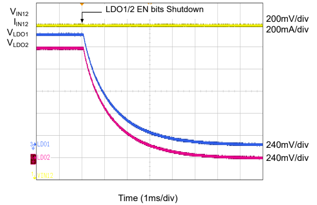
LDO1/2 EN bits Shutdown at I_{LDO1/2} = 0\text{mA}
