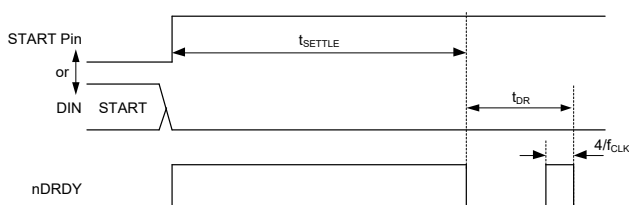
Figure 18. Settling Time
