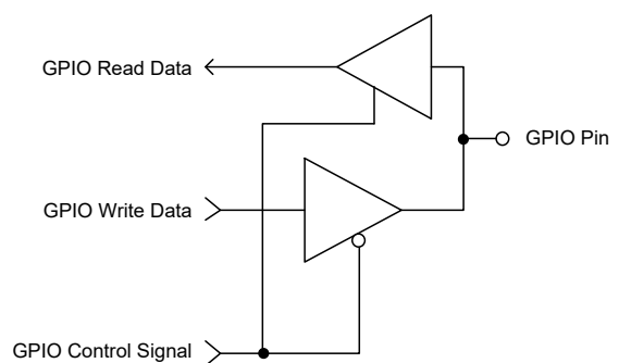
Figure 17. GPIO Pin Structure
