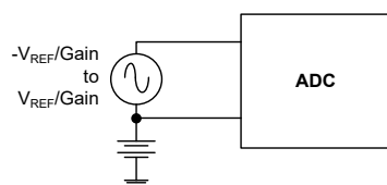
(a). Pseudo-Differential Input
