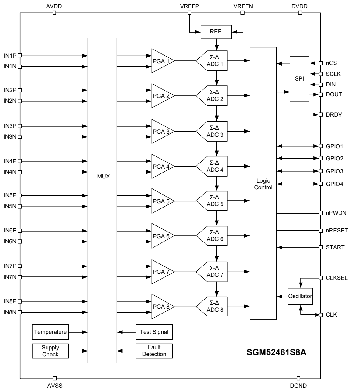
Figure 4. Block Diagram
