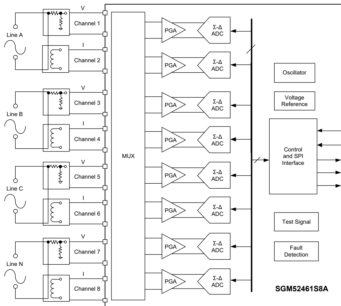
Figure 3. Simplified Schematic
