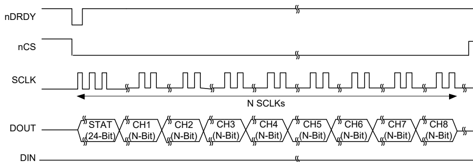
Figure 27. SGM52461S8A SPI Bus Data Output (Eight Channels)
