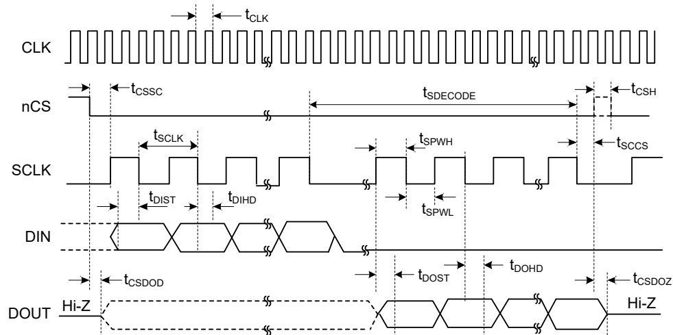
Figure 1. Serial Interface Timing Diagram
