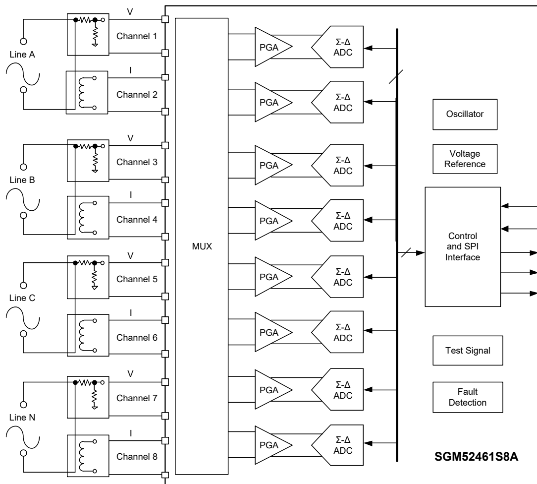
Figure 3. Simplified Schematic
