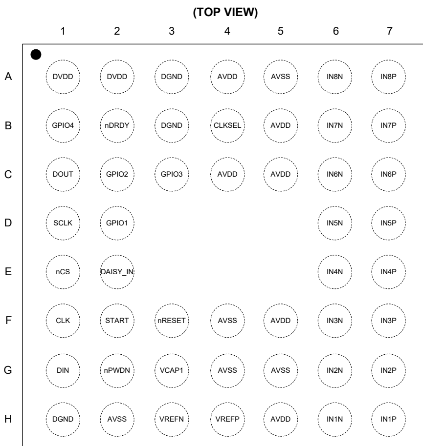
WLCSP-3.53×3.53-50B
