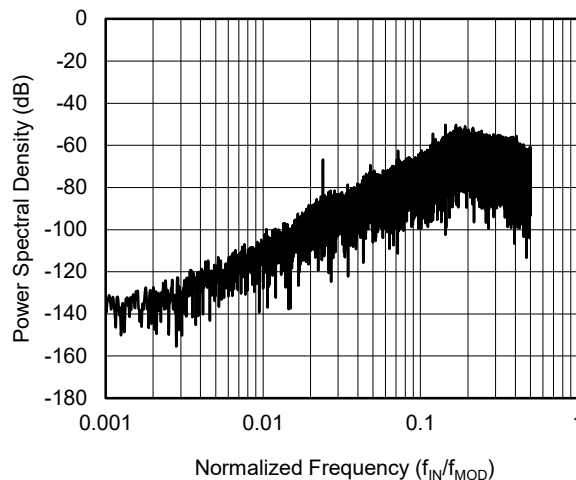
Figure 10. Modulator Noise Spectrum up to 0.5 \times f_{MOD}
