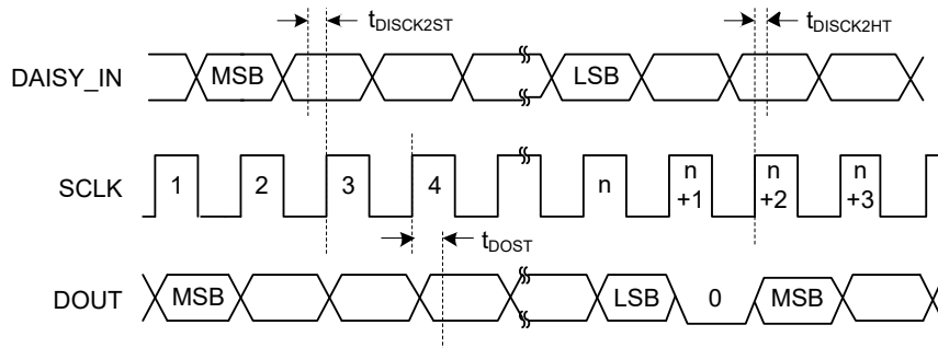
Figure 2. Daisy-Chain Interface Timing Diagram
