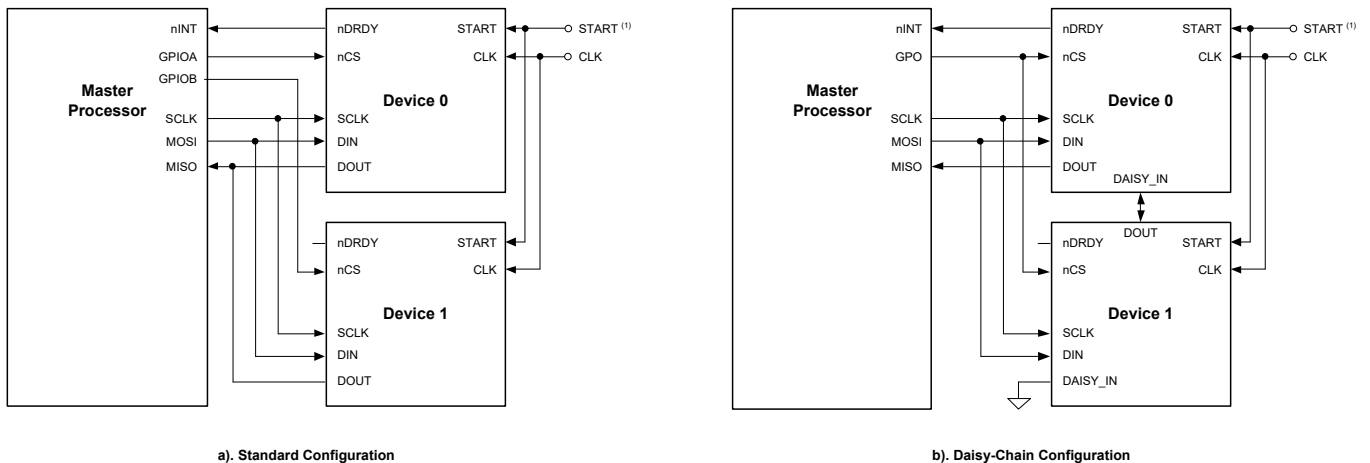
Figure 26. Multiple Device Configurations
