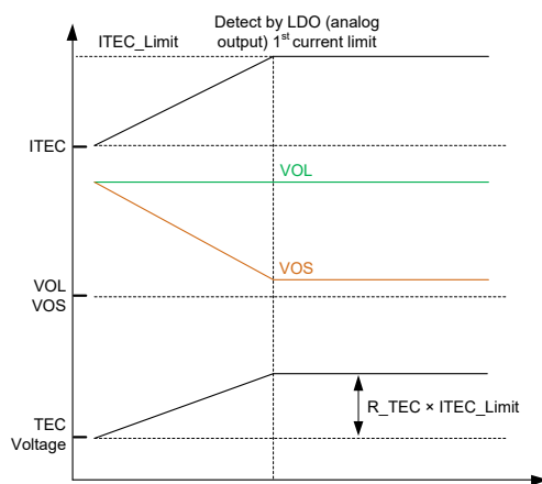
Figure 8. Primary Current Limit Protection (1 st Limit)
