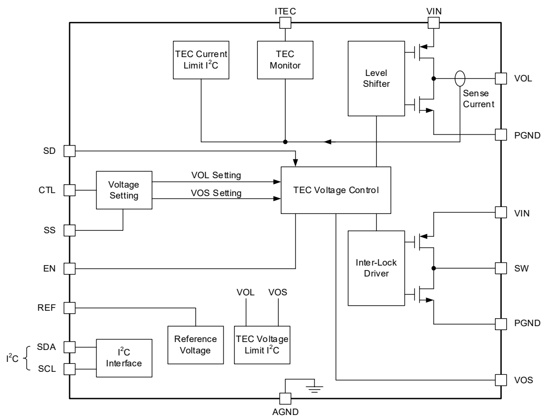
Figure 3. Block Diagram
