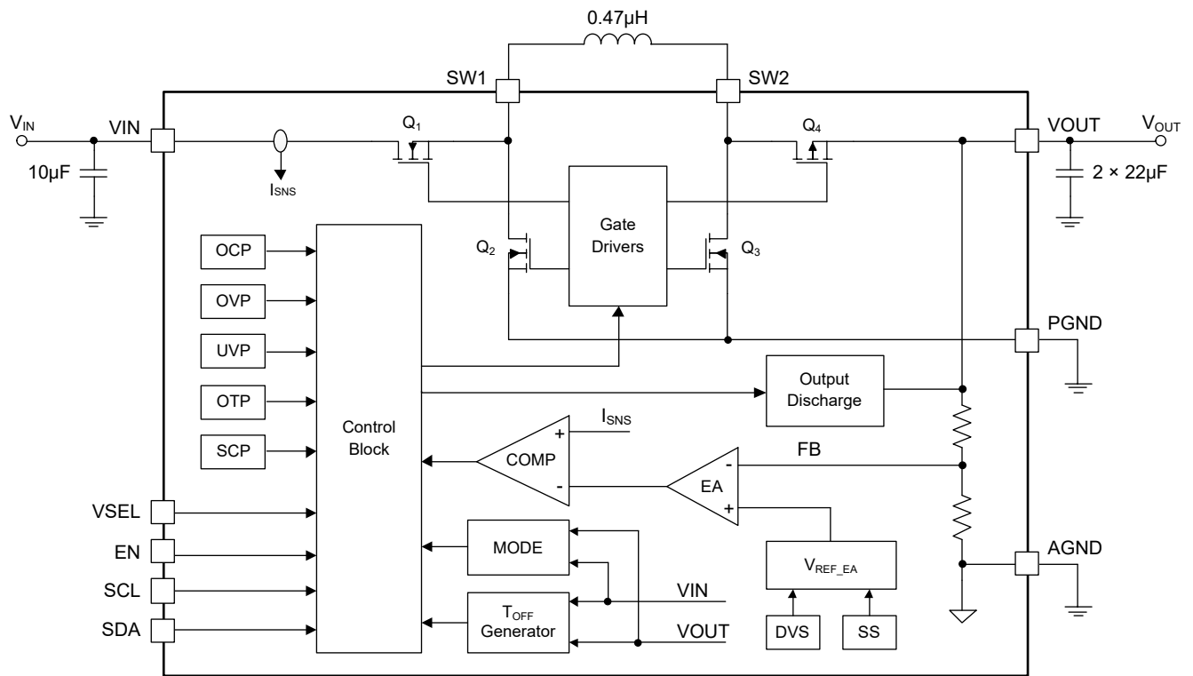
Figure 2. Block Diagram
