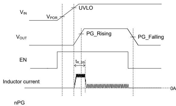
Figure 7. Startup Performance
