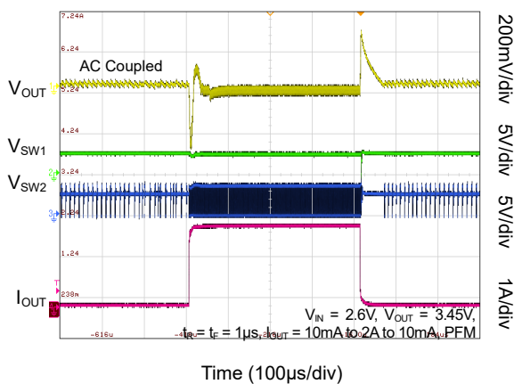
Load Transient Response in Boost Mode
