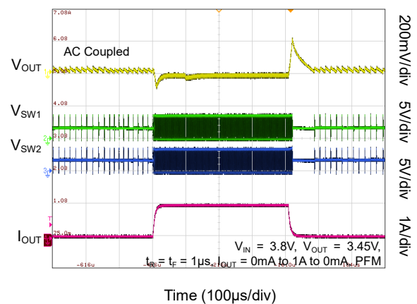
Load Transient Response (Typical Condition 1)
