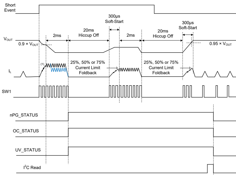
Figure 11. Short-Circuit Protection
