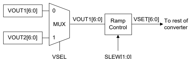
Figure 9. Block Diagram of the Dynamic Voltage Scaling
