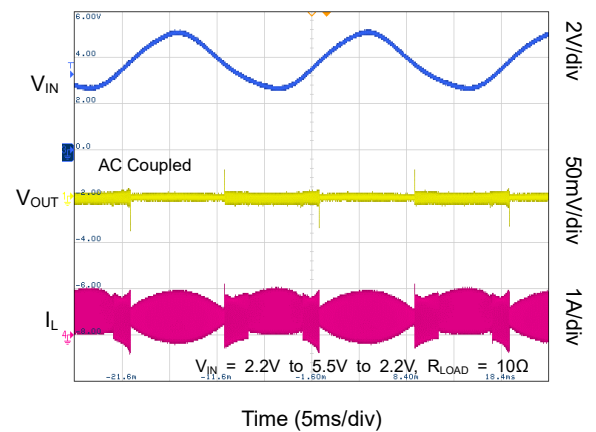
Line Sweep under FPWM
