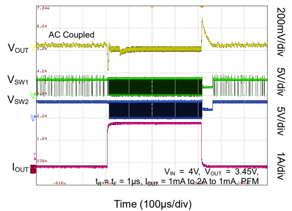
Load Transient Response (Typical Condition 3)
