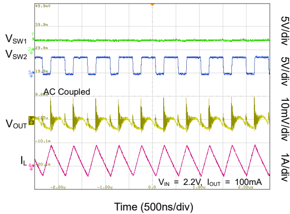
FPWM Switching Waveforms in Boost Mode
