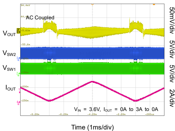
Load Sweep under PFM
