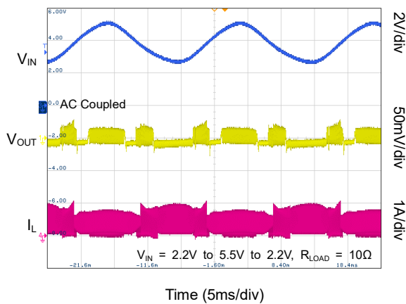
Line Sweep under PFM
