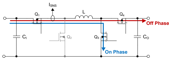
Figure 4. Boost Mode Switching
