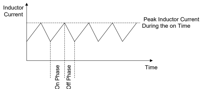
Figure 5. Buck or Boost Mode Peak Current Control
