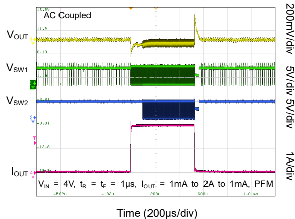
Load Transient Response (Typical Condition 2)
