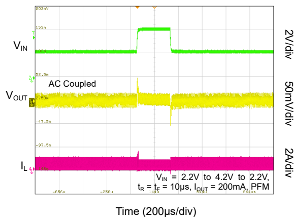
Line Transient Response under Light Load
