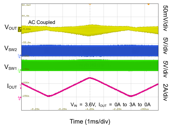
Load Sweep under FPWM
