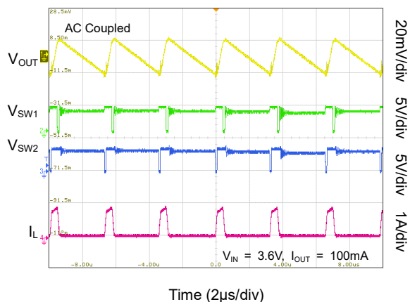
PFM Switching Waveforms in Buck-Boost Mode
