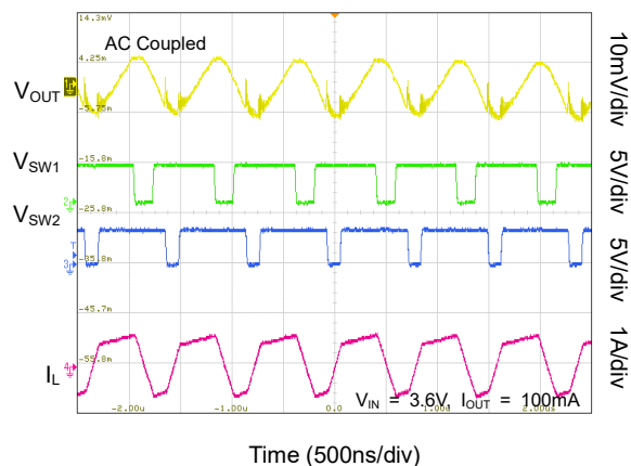
FPWM Switching Waveforms in Buck-Boost Mode
