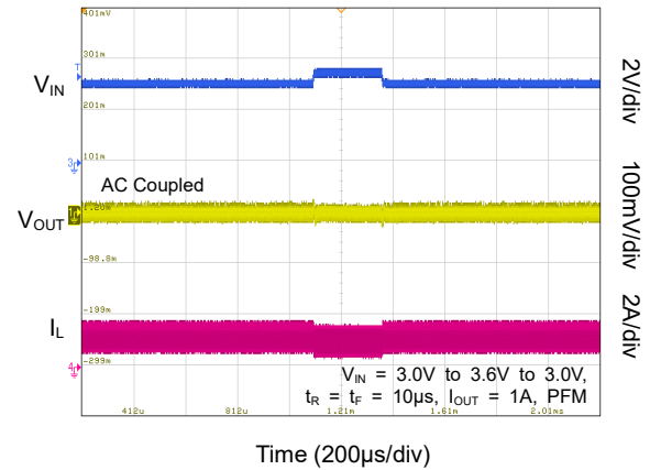
Line Transient Response (Typical Condition)
