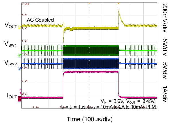
Load Transient Response in Buck-Boost Mode
