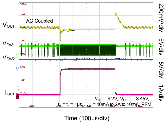
Load Transient Response in Buck Mode
