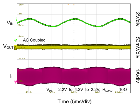
Line Sweep under FPWM
