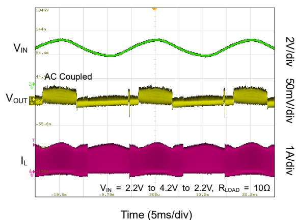
Line Sweep under PFM
