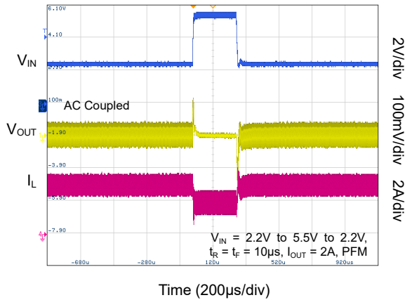
Line Transient Response under Heavy Load
