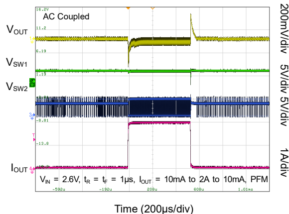
Load Transient Response in Boost Mode
