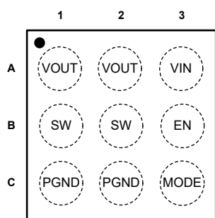
WLCSP-1.20x1.21-9B
