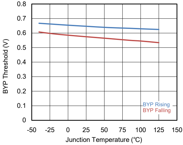
BYP Threshold vs. Temperature
