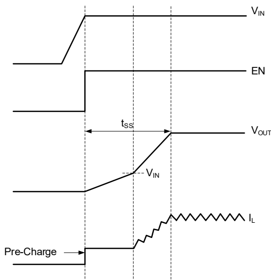
Figure 3. Startup Sequence
