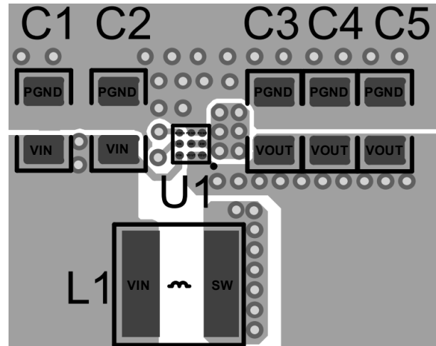
Figure 6. SGM66155 PCB Layout
