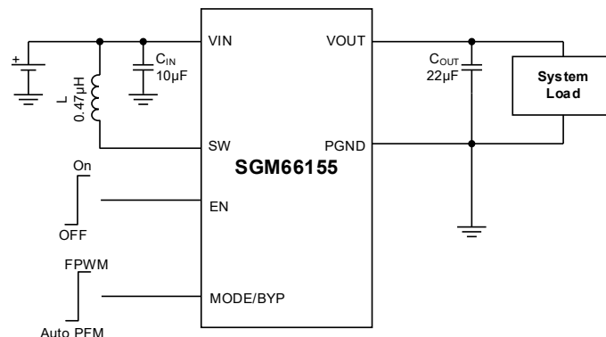
Figure 1. Simplified Schematic
