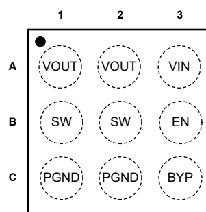
WLCSP-1.20x1.21-9B
