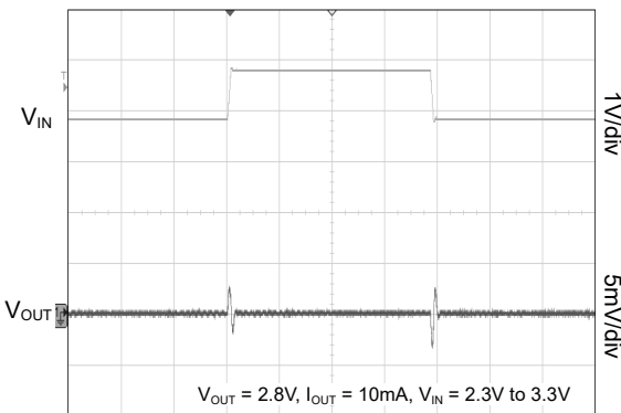
Time (20µs/div)
