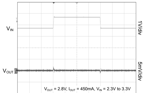
Time (20µs/div)
