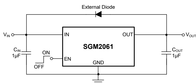
Figure 4. Reverse Protection Reference Design
